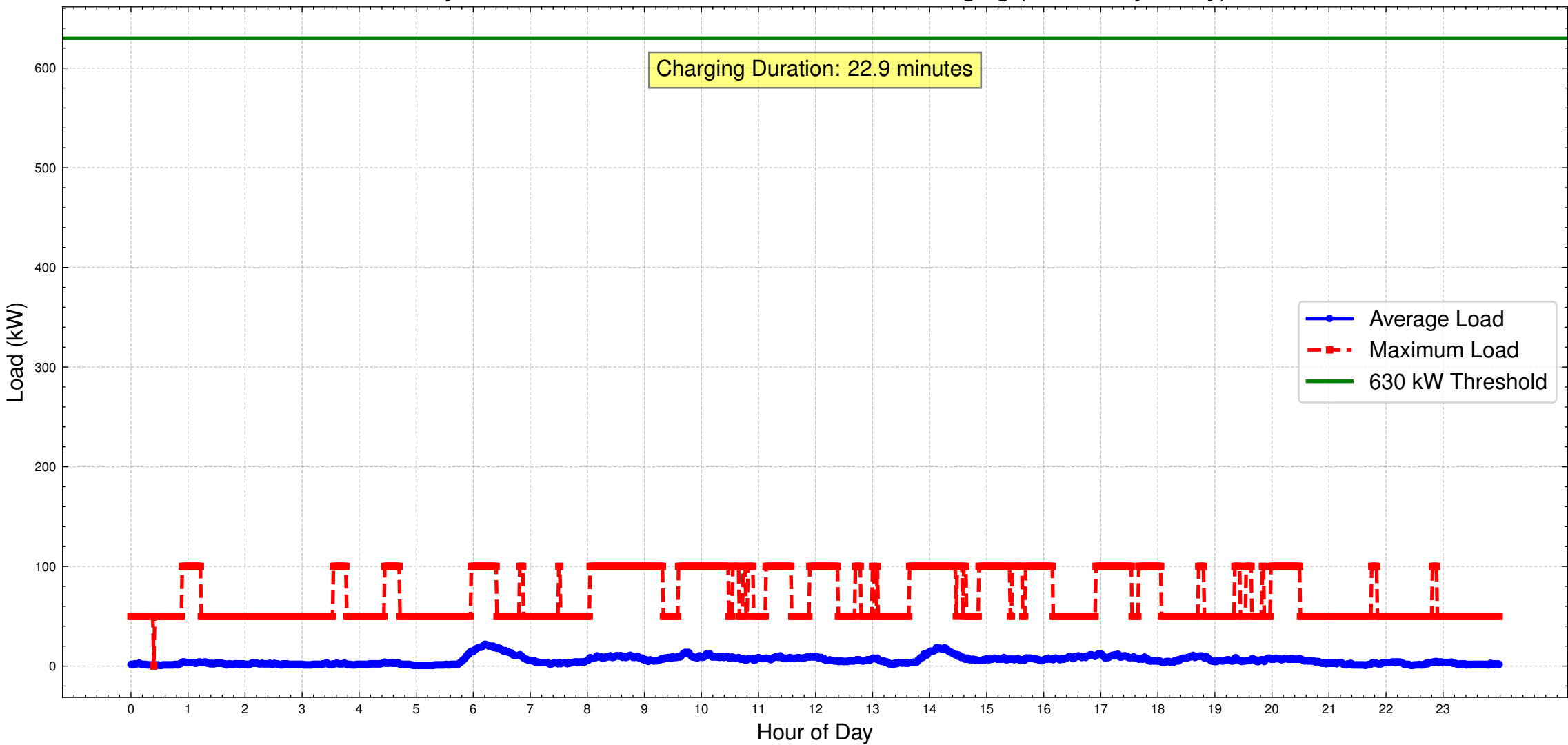
Daily Load Profile for Base 1251 with 50 kW Charging (Active Days Only)
