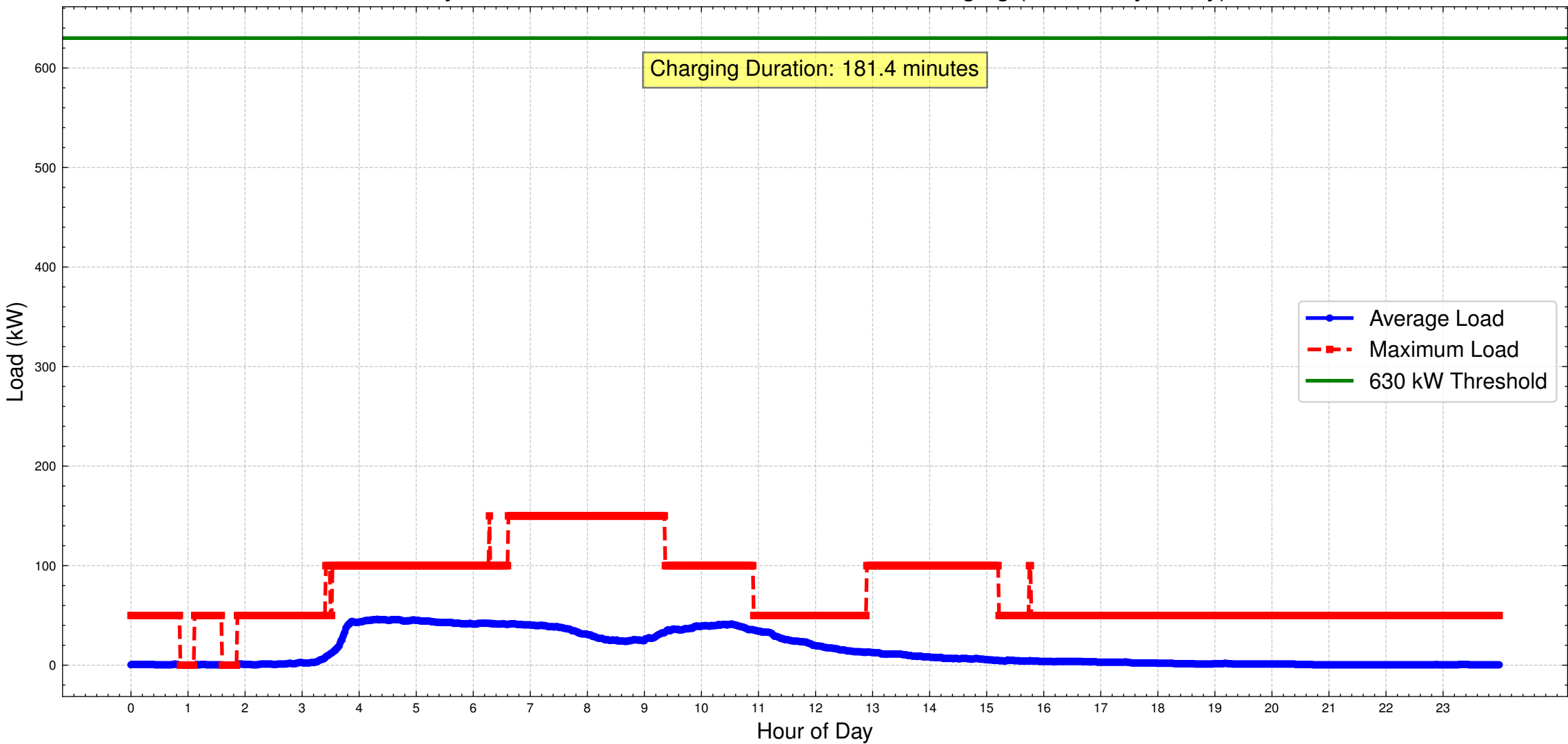
Daily Load Profile for Base 1265 with 50 kW Charging (Active Days Only)
