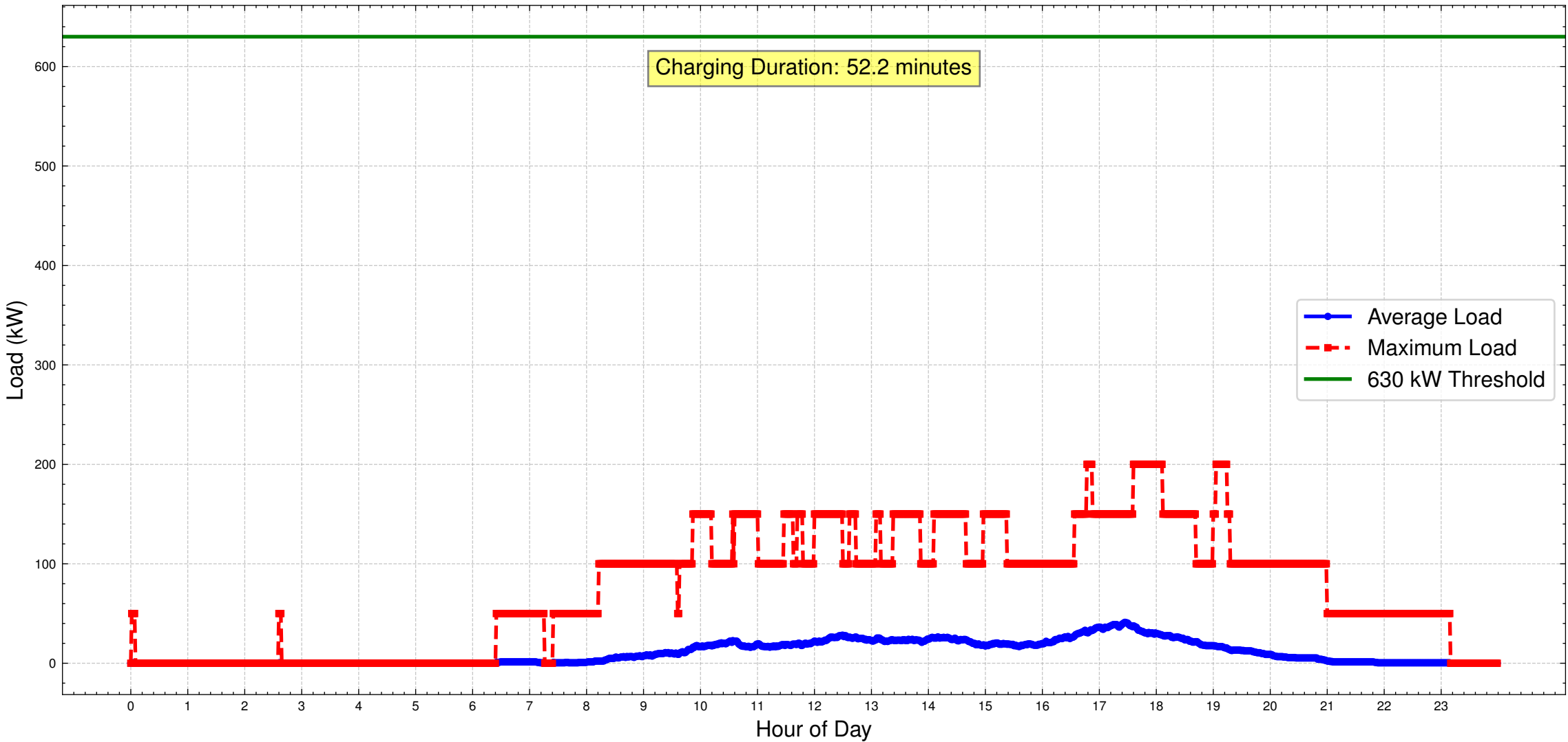
Daily Load Profile for Base 2 with 50 kW Charging (Active Days Only)
