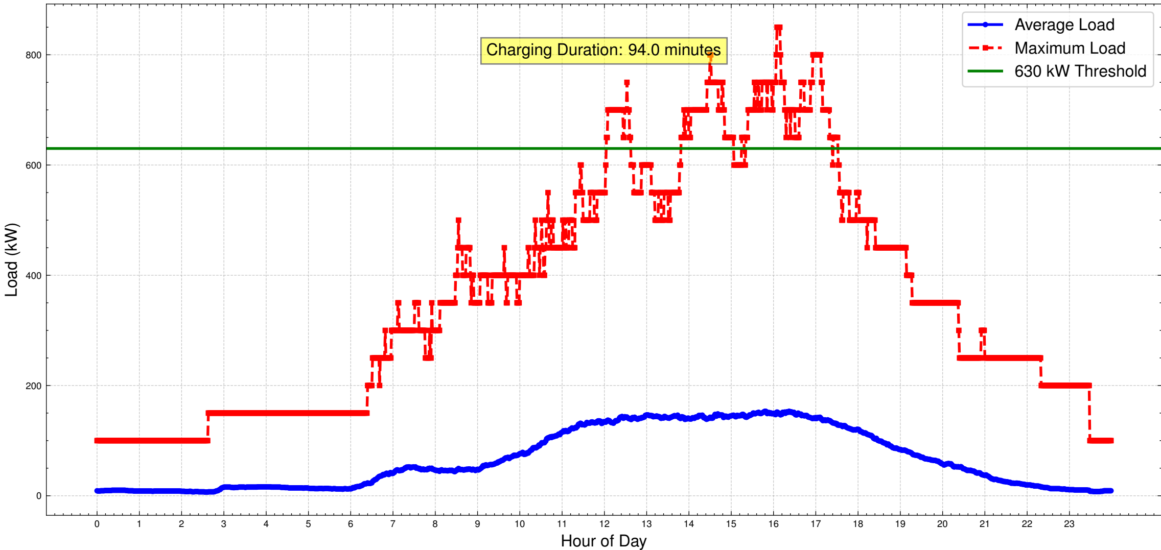
Daily Load Profile for Base 412 with 50 kW Charging (Active Days Only)
