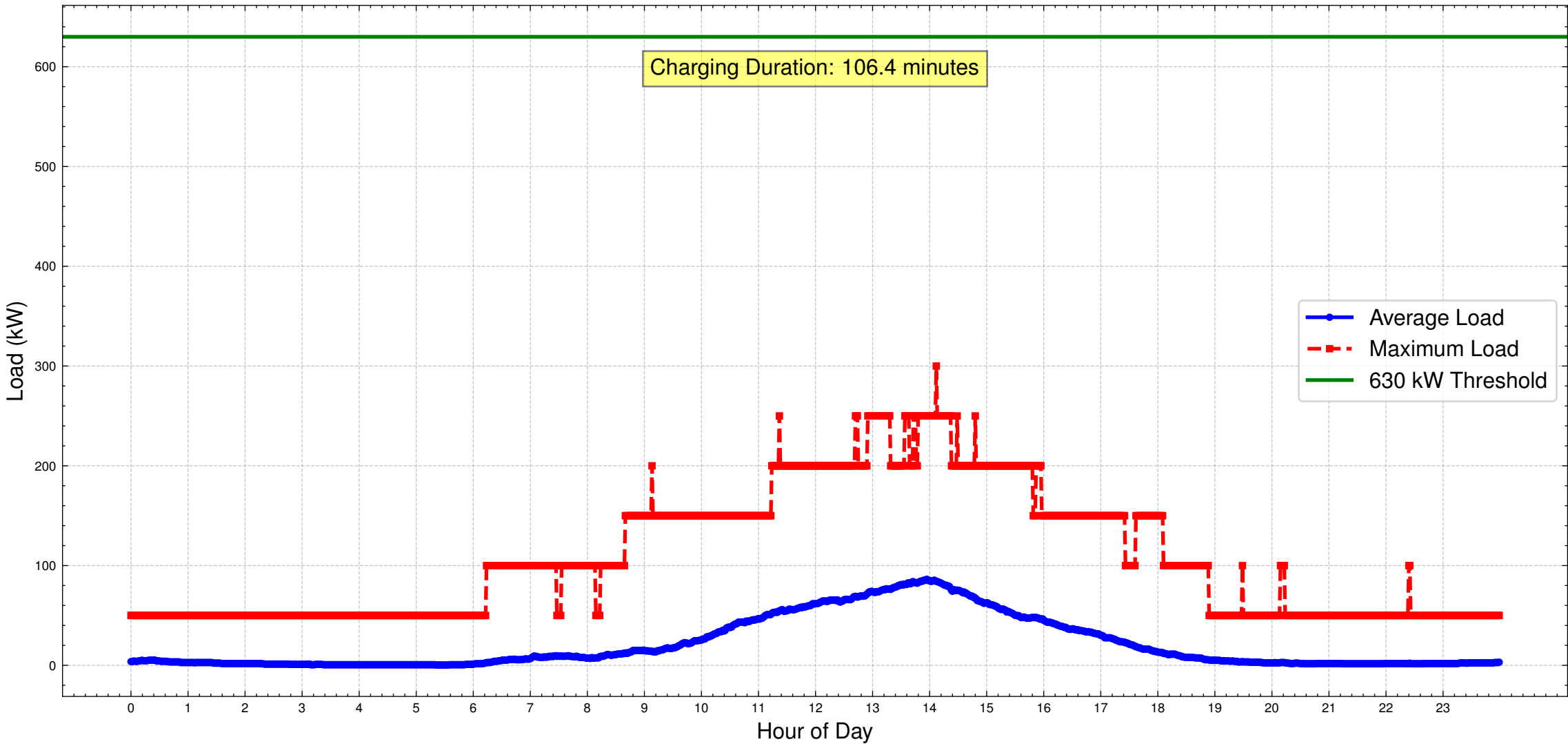
Daily Load Profile for Base 745 with 50 kW Charging (Active Days Only)
