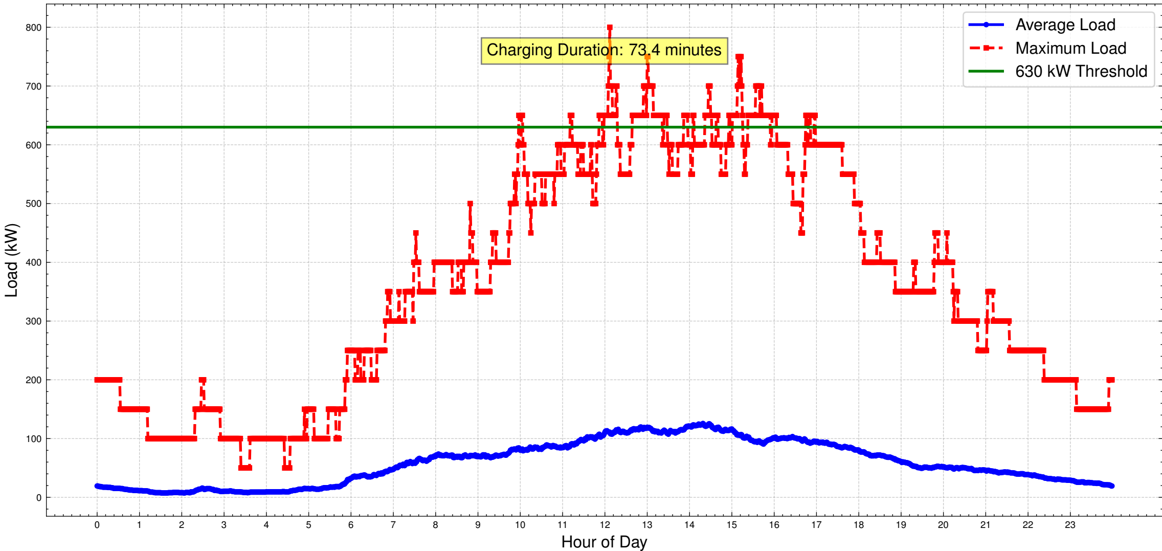
Daily Load Profile for Base 809 with 50 kW Charging (Active Days Only)
