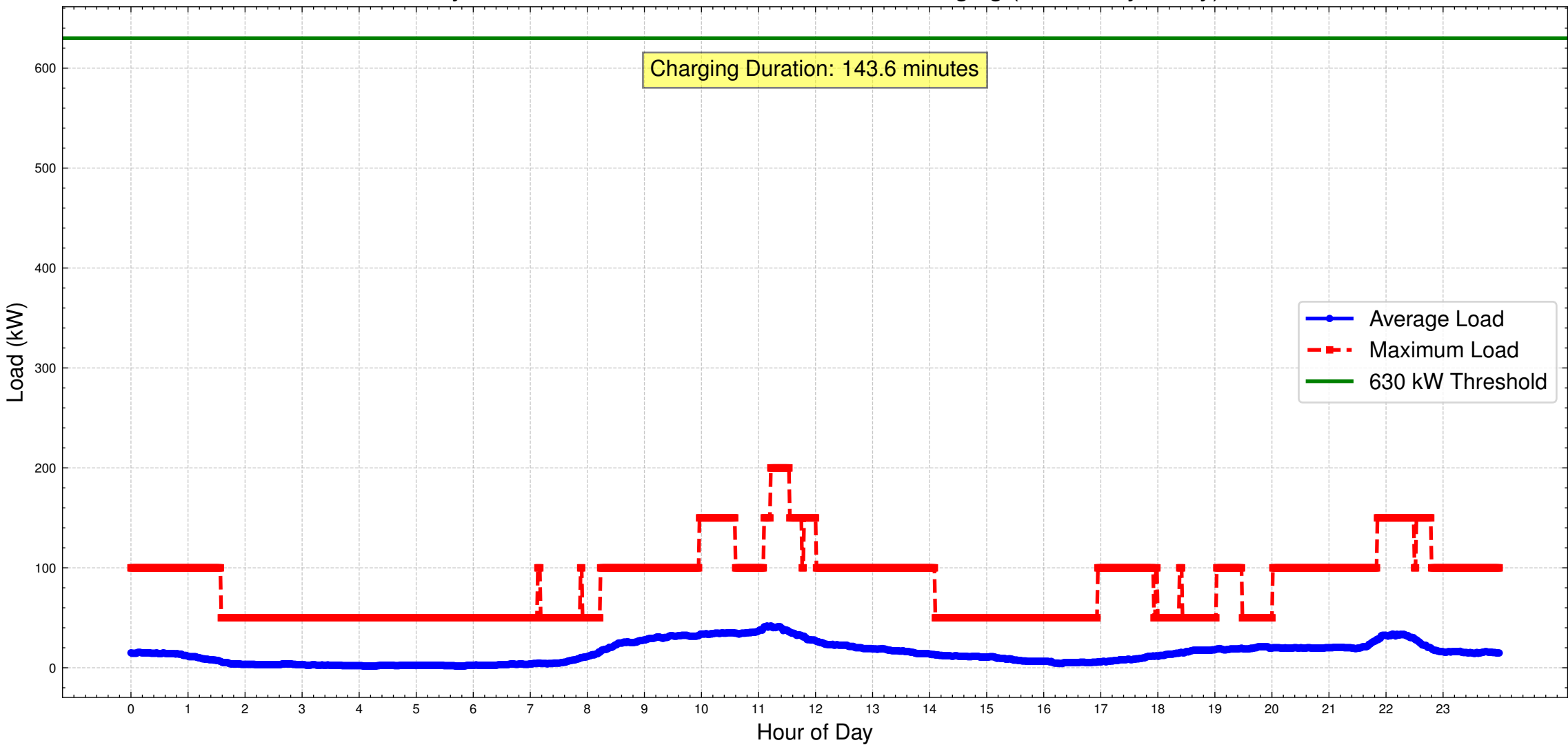
Daily Load Profile for Base 868 with 50 kW Charging (Active Days Only)
