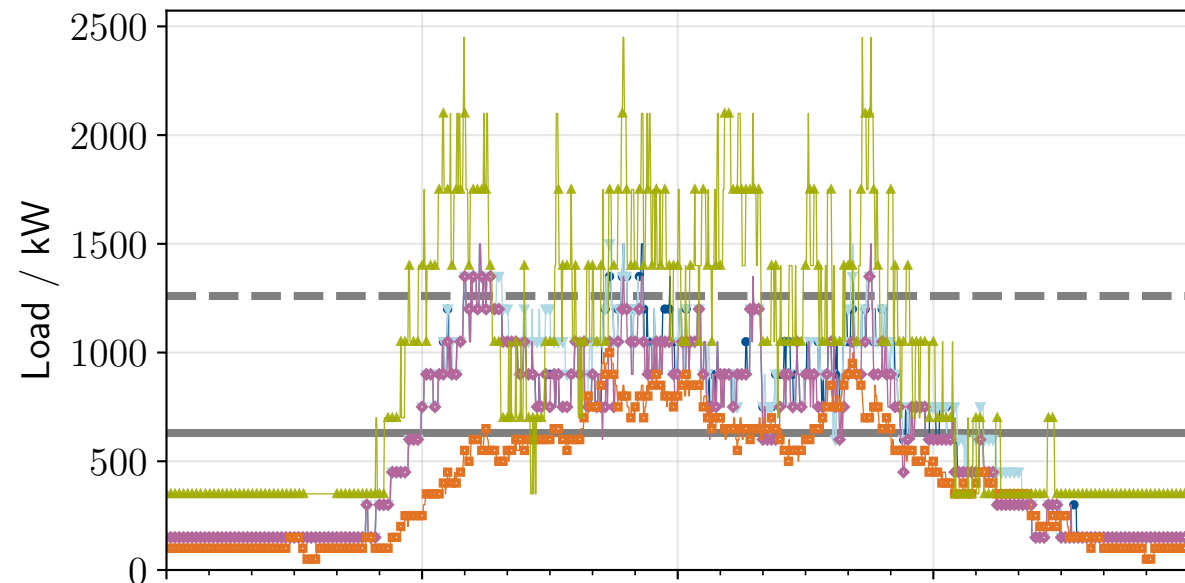
Location CID-412: Maximum Load Profile
