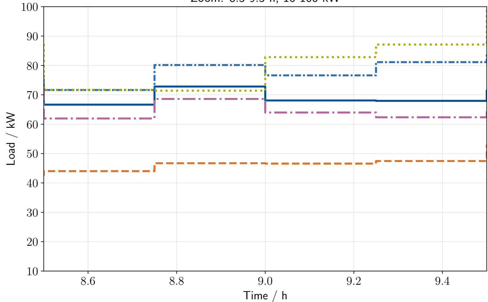
Location CID-842: 15-Minute Average Load Zoom: 8.5-9.5 h, 10-100 kW
