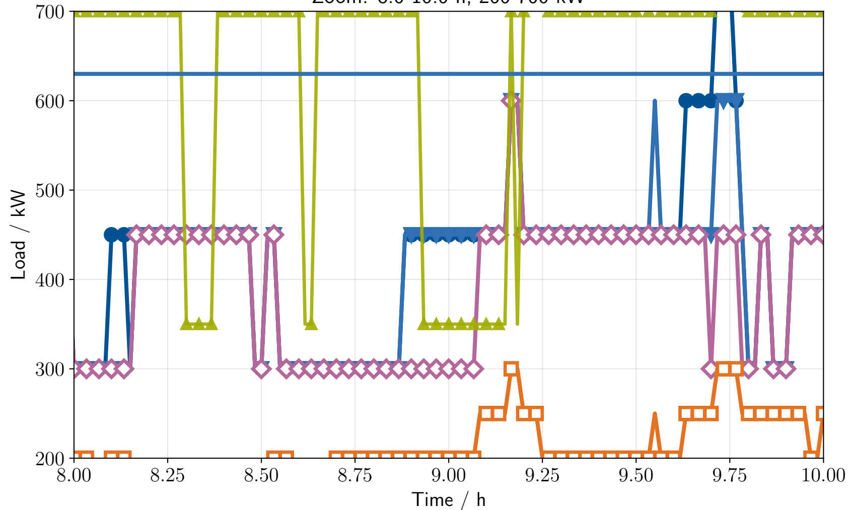
Location CID-842: Maximum Load Profile Zoom: 8.0-10.0 h, 200-700 kW
