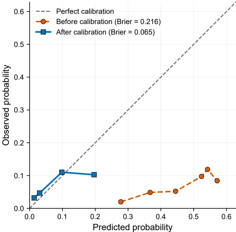
Calibration Curve of the XGBoost Prediction Model
