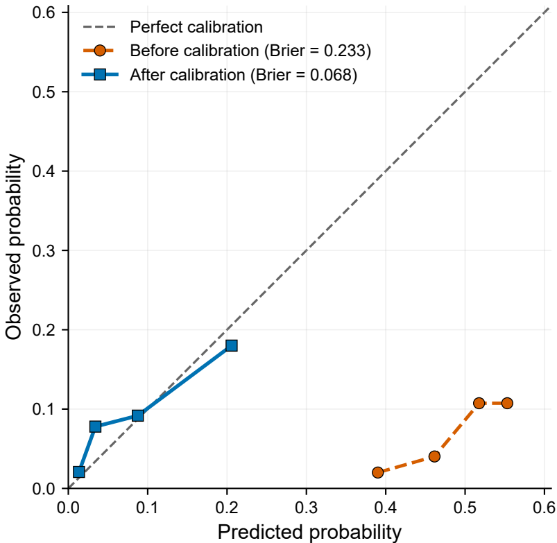
Calibration Curve of the CatBoost Prediction Model
