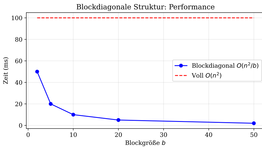
Abbildung 16.8: Experiment 5: Block-Diagonal Performance
