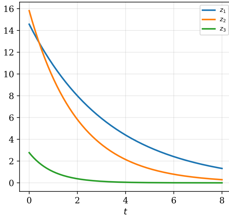
Modalkoordinaten \dot{\mathbf{z}} = \mathbf{J}\mathbf{z}, \mathbf{z} = \mathbf{V}^{-1}\mathbf{x}
