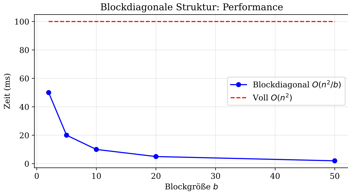
Abbildung 16.8: Experiment 5: Block-Diagonal Performance
