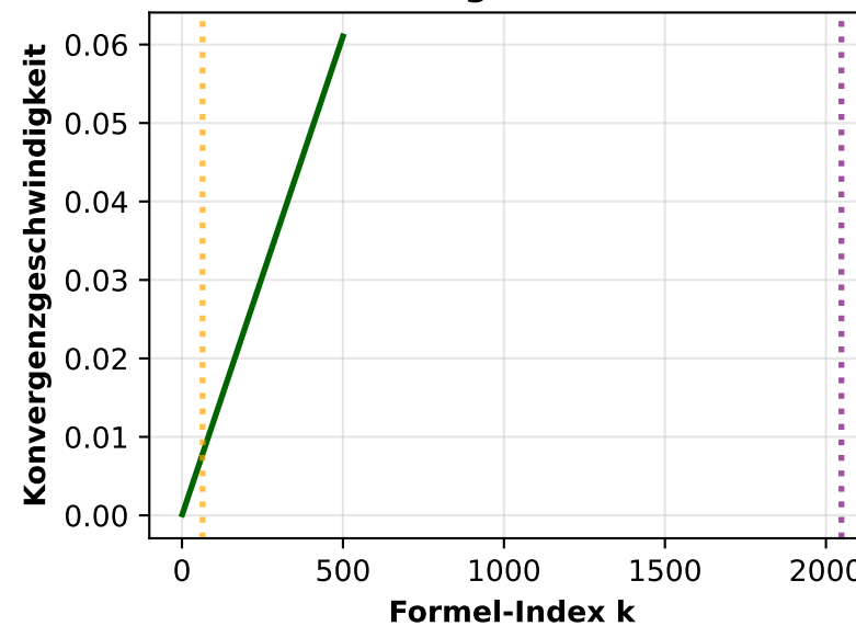
n = 12: Konvergenz zu Worst-Case
