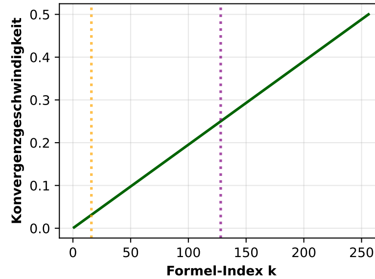
n = 8: Konvergenz zu Worst-Case
