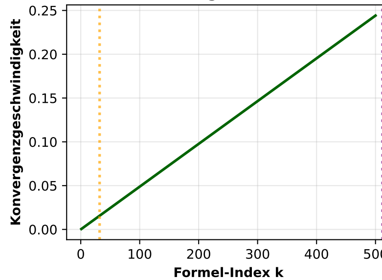
n = 10: Konvergenz zu Worst-Case
