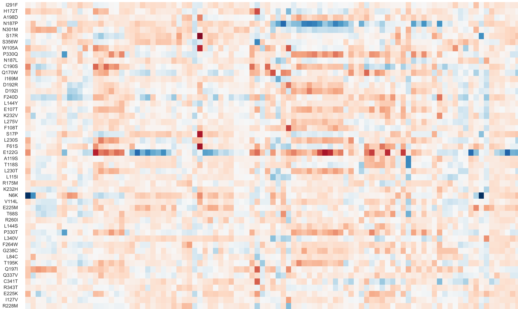
ADRB2_HUMAN_Jones_2020 — top 50 variants by disagreement
