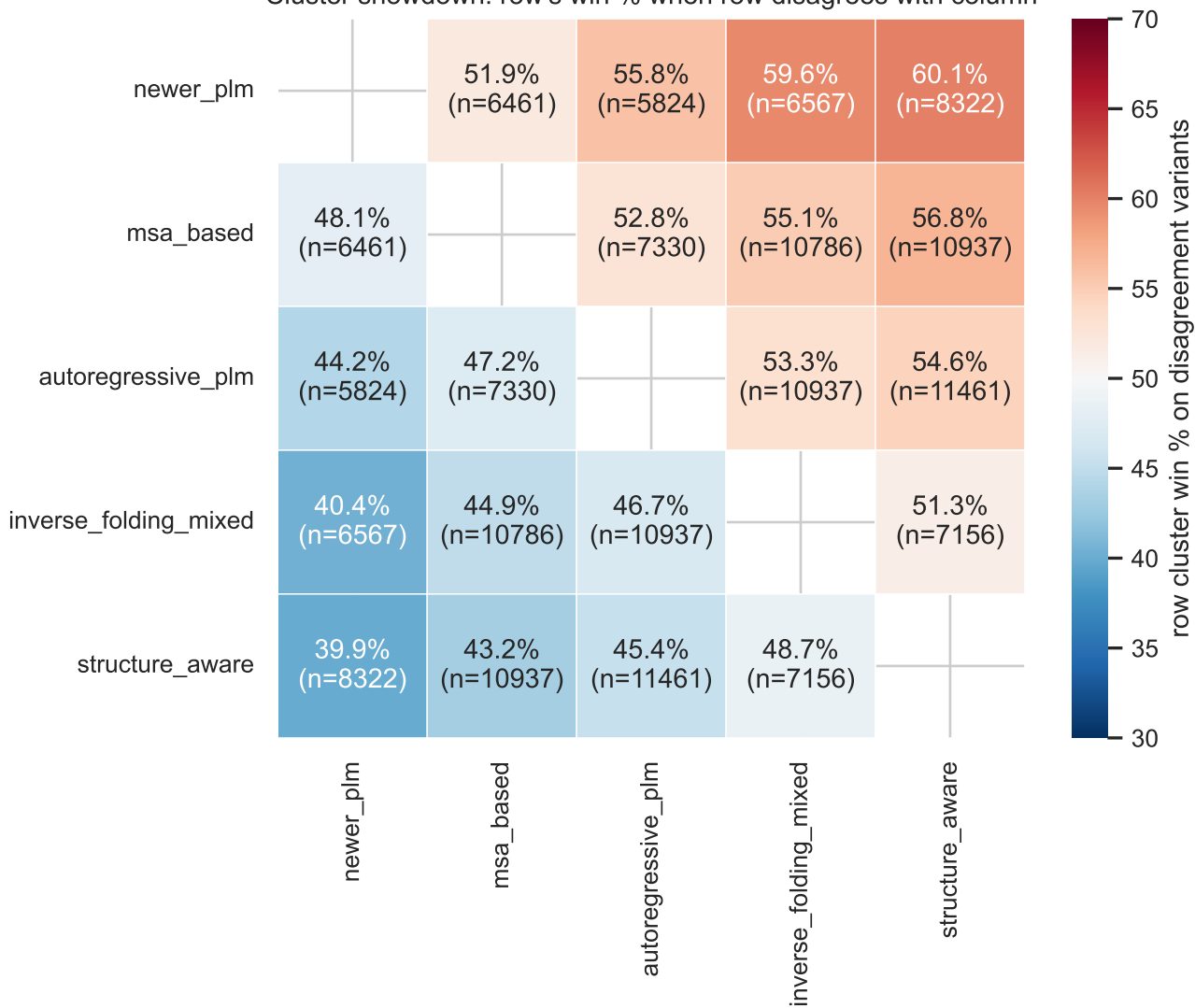
Cluster showdown: row's win % when row disagrees with column
