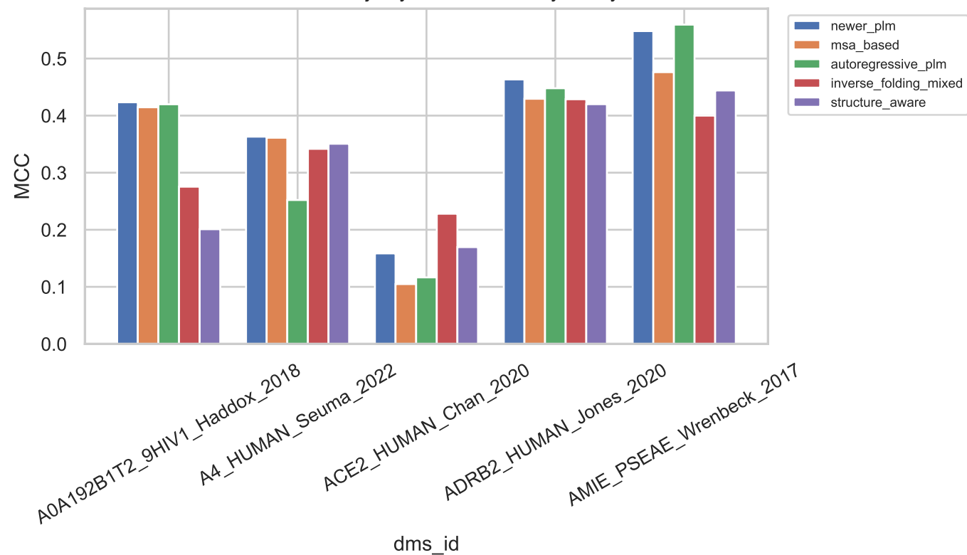
Per-cluster majority-vote MCC — by assay
