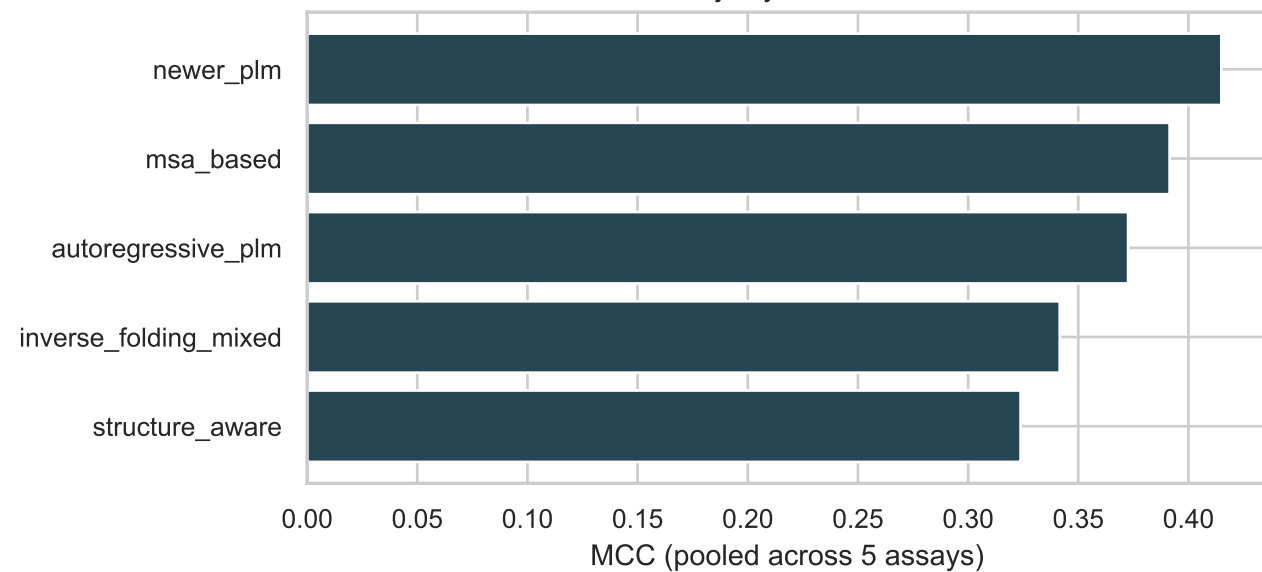
Per-cluster majority-vote MCC — overall
