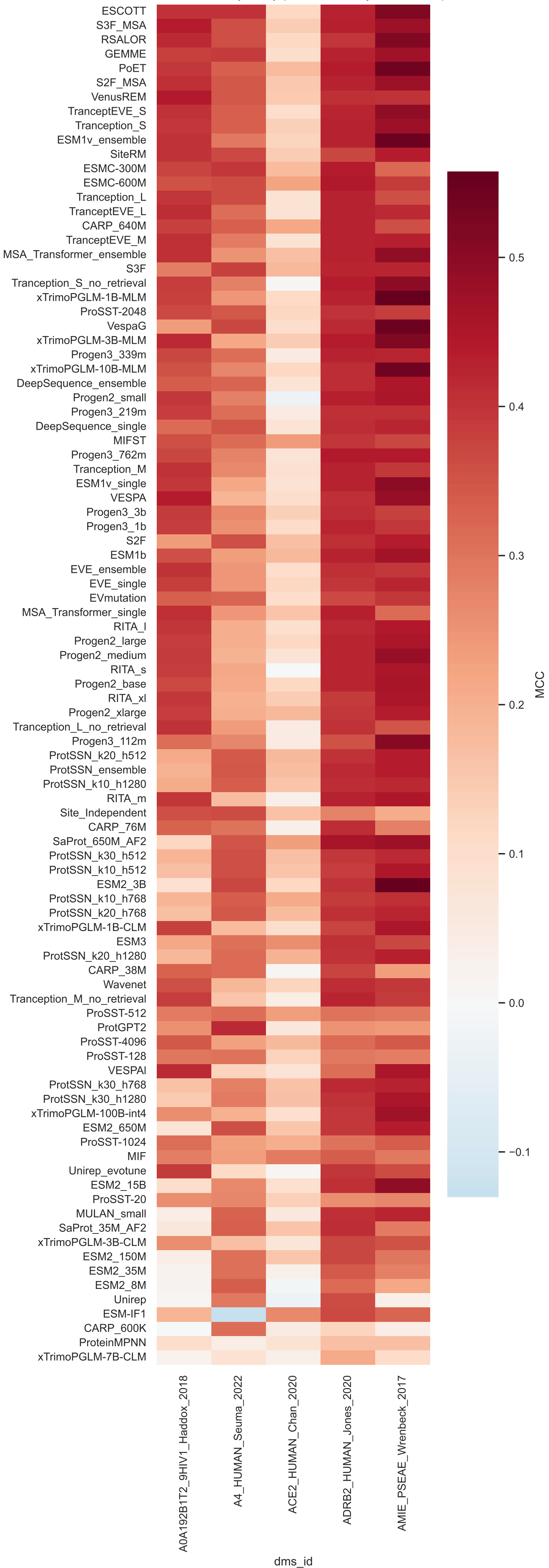
Per-model MCC by assay (rows ordered by overall MCC)
