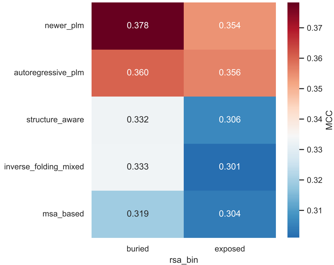
Cluster MCC by burial (RSA bin)
