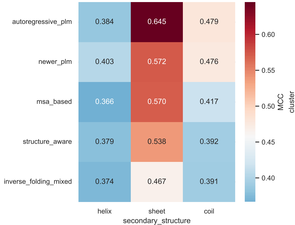
Cluster MCC by secondary structure
