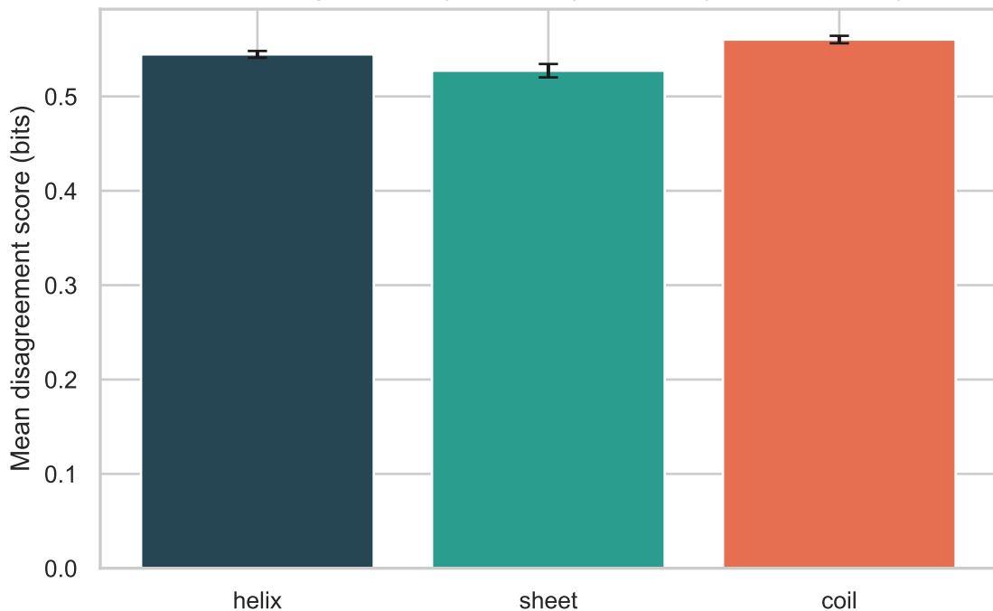
Mean disagreement by secondary structure (pooled, +/- SEM)
