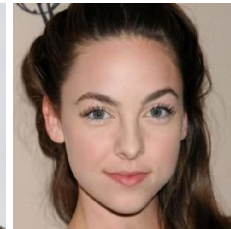
Nearest train
