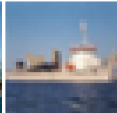
Nearest train
