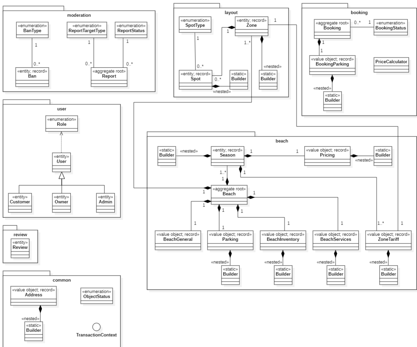
Figura 7: Domain UML
