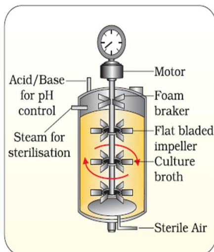
Simple stirred-tank
