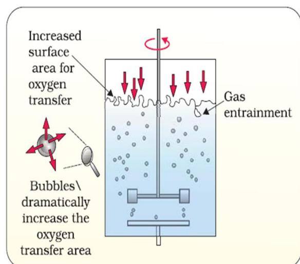
Sparged stirred-tank bioreactor through which sterile air bubbles are sparged
