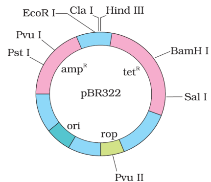
Figure: E. coli cloning vector pBR322 showing restriction sites (Hind III, EcoR I, BamH I, Sal I, Pvu II, Pst I, Cla I), ori and antibiotic resistance genes ( amp^R and tet^R ). Rop codes for the proteins involved in the replication of the plasmid
