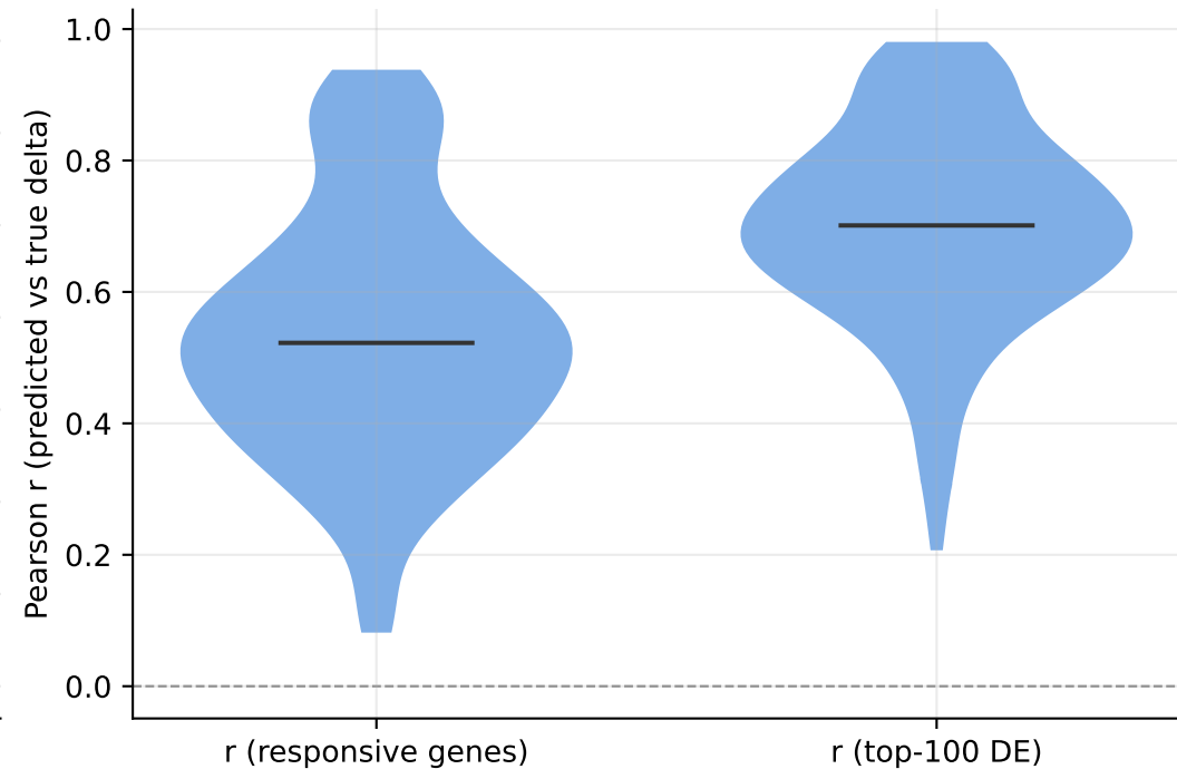
B Pseudobulk delta accuracy
