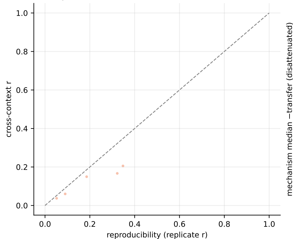
B Why raw correlation misleads (rho=+1.00)
