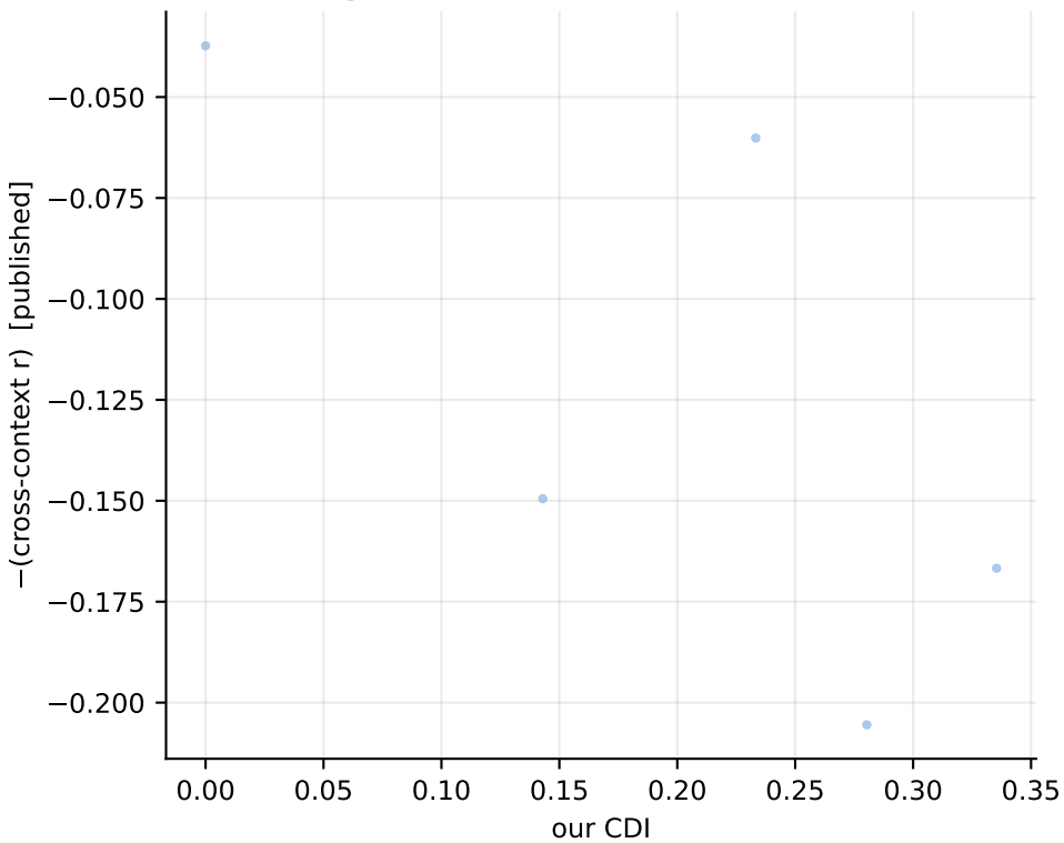
A Ours vs published (rho=-0.80)
