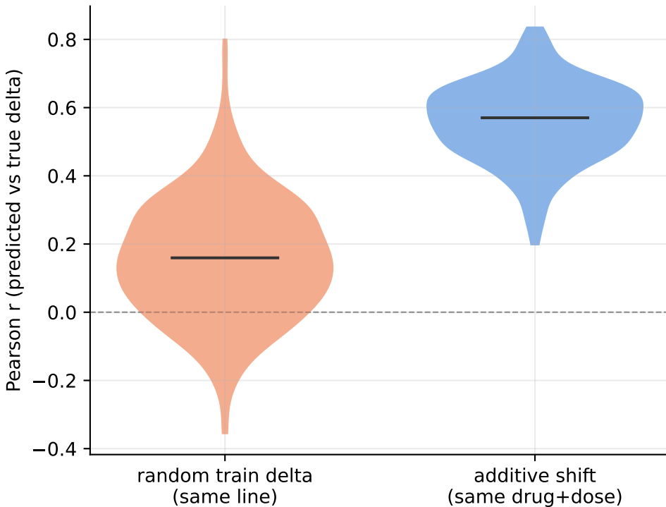
A r on 2,000 most responsive genes
