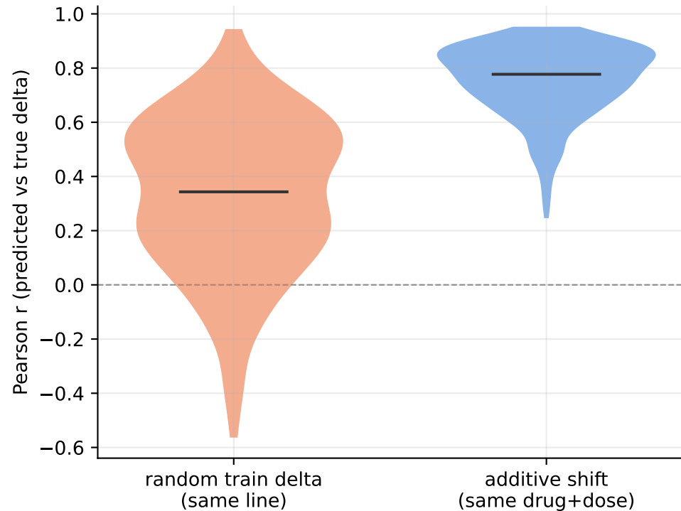
B r on condition's top-100 DE genes
