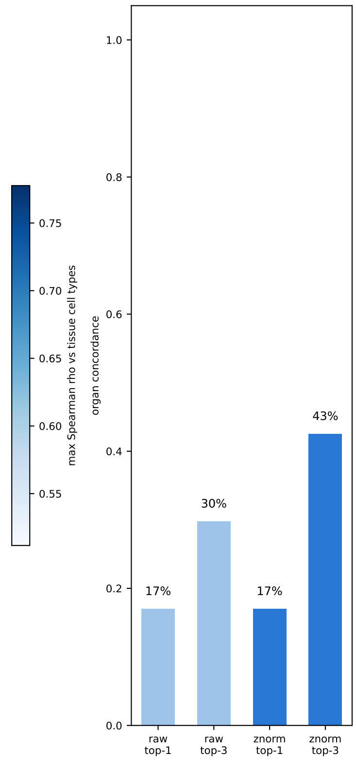
B Concordance
