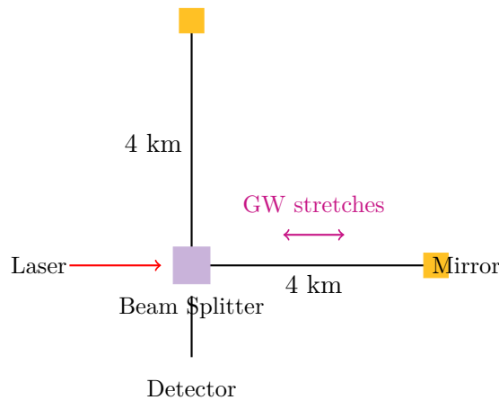
Figure 10: Simplified LIGO interferometer schematic. Gravitational waves stretch one arm while compressing the other.
