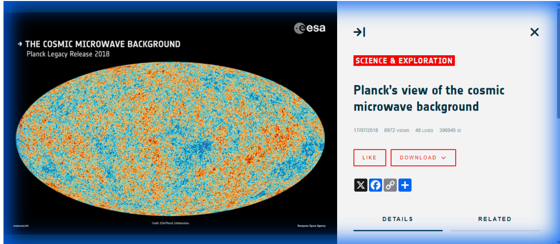
Figure 9: Planck satellite all-sky map of CMB temperature anisotropies. Red regions are \sim 0.0001 K warmer than average; blue regions are cooler. These tiny fluctuations grew into all cosmic structure.
