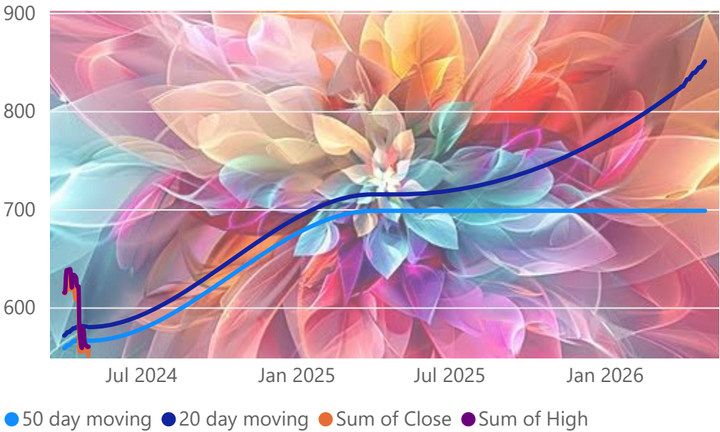
50 day moving, 20 day moving, Sum of Close and Sum of High by Date
