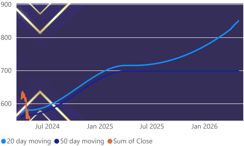
20 day moving, 50 day moving and Sum of Close by Date
