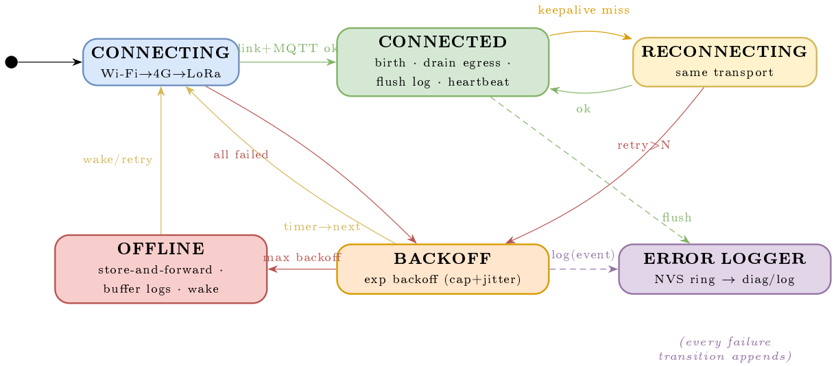
Figure 11: Link Manager FSM: transport failover, backoff, and an error logger that flushes the NVS ring to diag/log when CONNECTED (so offline faults still reach the cloud).
