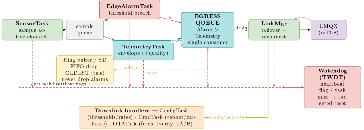
Figure 10: Runtime FreeRTOS tasks, priority egress queue, store-and-forward, downlink handlers and heartbeat watchdog.
