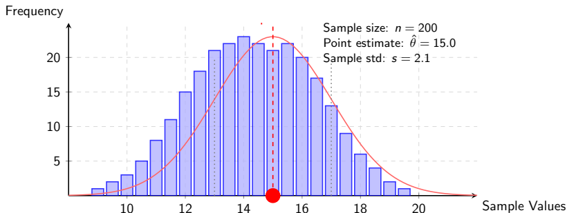
Figure: Sample histogram with point estimate \hat{\theta} showing the center of the distribution
