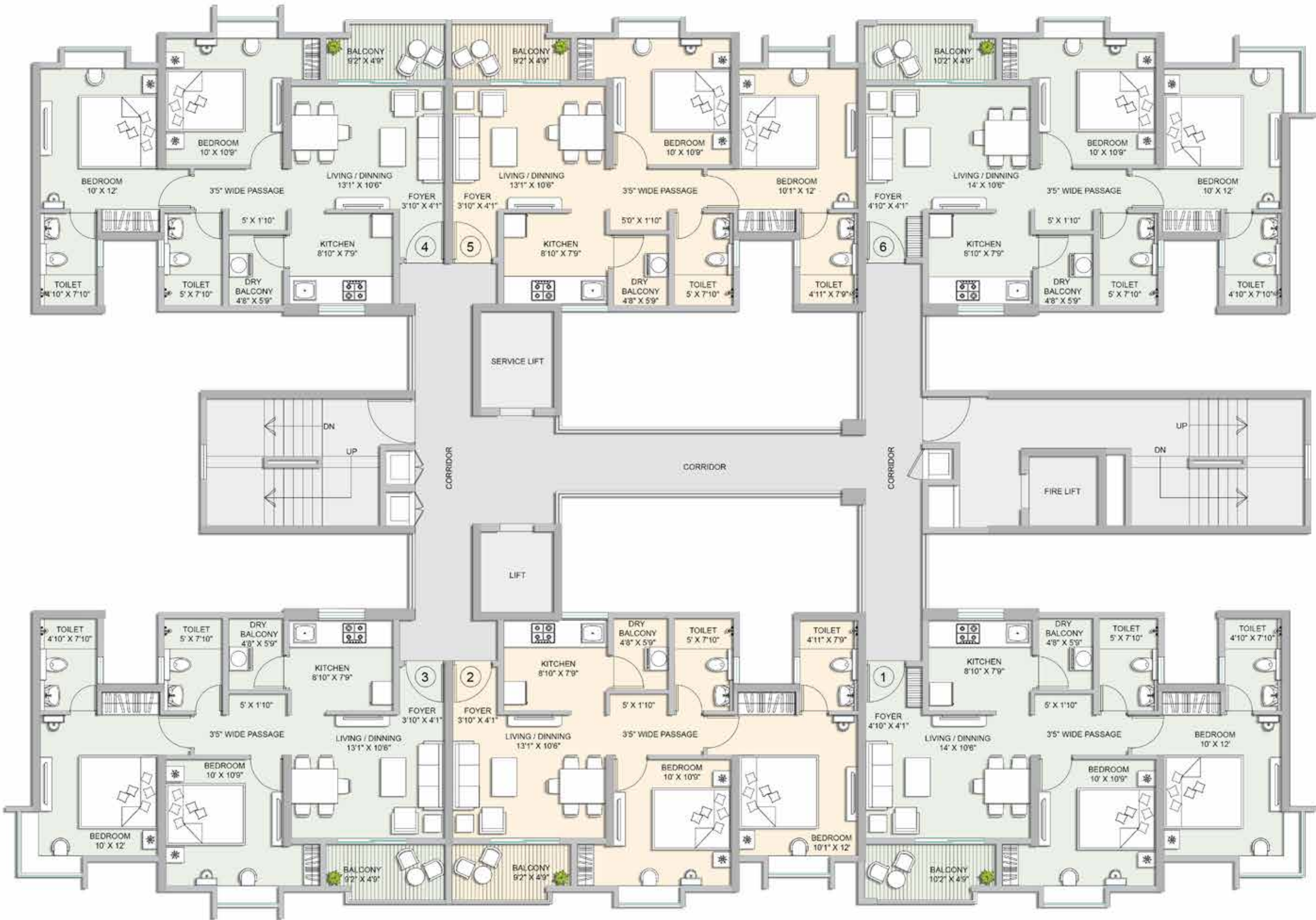
TOWER NT4 (AMBER) 1ST,3RD,5TH,7TH,9TH,&11TH,15TH,17TH,21ST,23RD ODD FLOOR PLAN
