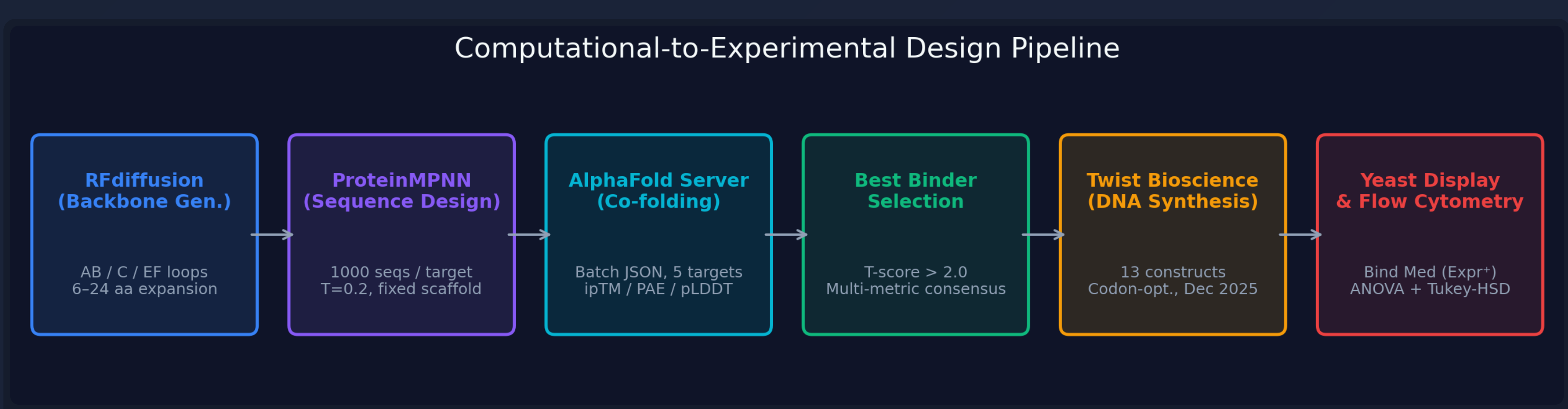
Figure 2: Six-stage generative-AI-to-experiment pipeline. Backbone generation (RFdiffusion) → sequence design (ProteinMPNN) → structural co-folding (AlphaFold3) → T-score candidate selection → DNA synthesis → yeast surface display & flow cytometry. Reduces >1,000 generated sequences to 13 synthesis-ready constructs.
