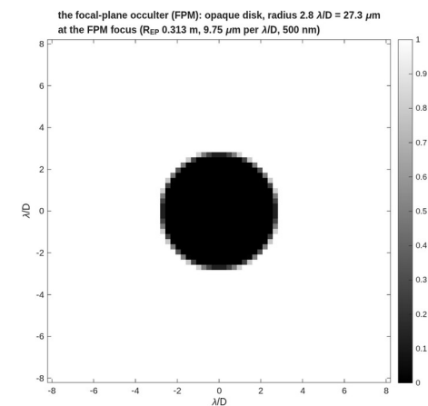
The focal-plane occulter, transmission against \lambda/D ; the physical radius is stated on the figure.
