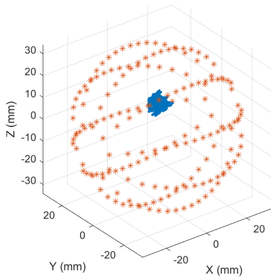
DDScat with 180to
