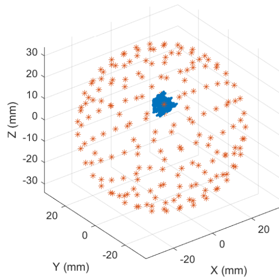
DDScat with 231to
