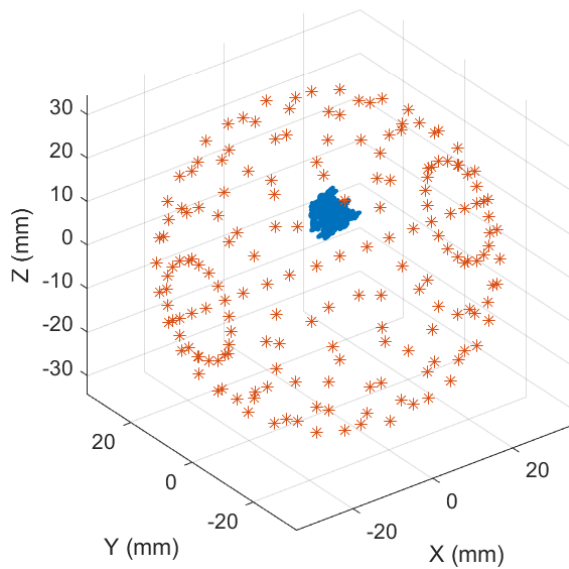
NESCoP with aq231id
