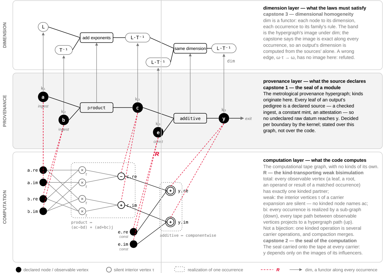
Figure 3. The three layers and their two ladders, drawn on the module y = a \cdot b + e at three granularities.
