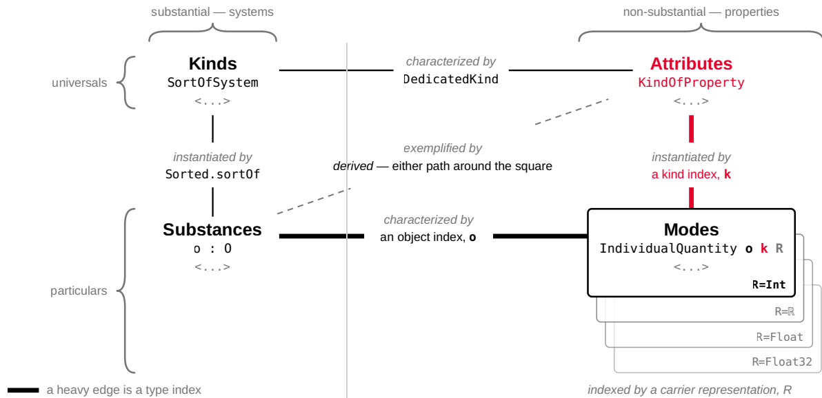
Figure 1. Lowe's ontological square with the calculus's identifiers at its corners and its mechanisms on its edges. The two heavy edges are the two type indices of an individual quantity — the object index o along the bottom and the kind index k down the right — and the plates behind the Modes corner are the carrier R , which indexes that corner alone. Each corner's instance slot is left empty; a model fills it.
