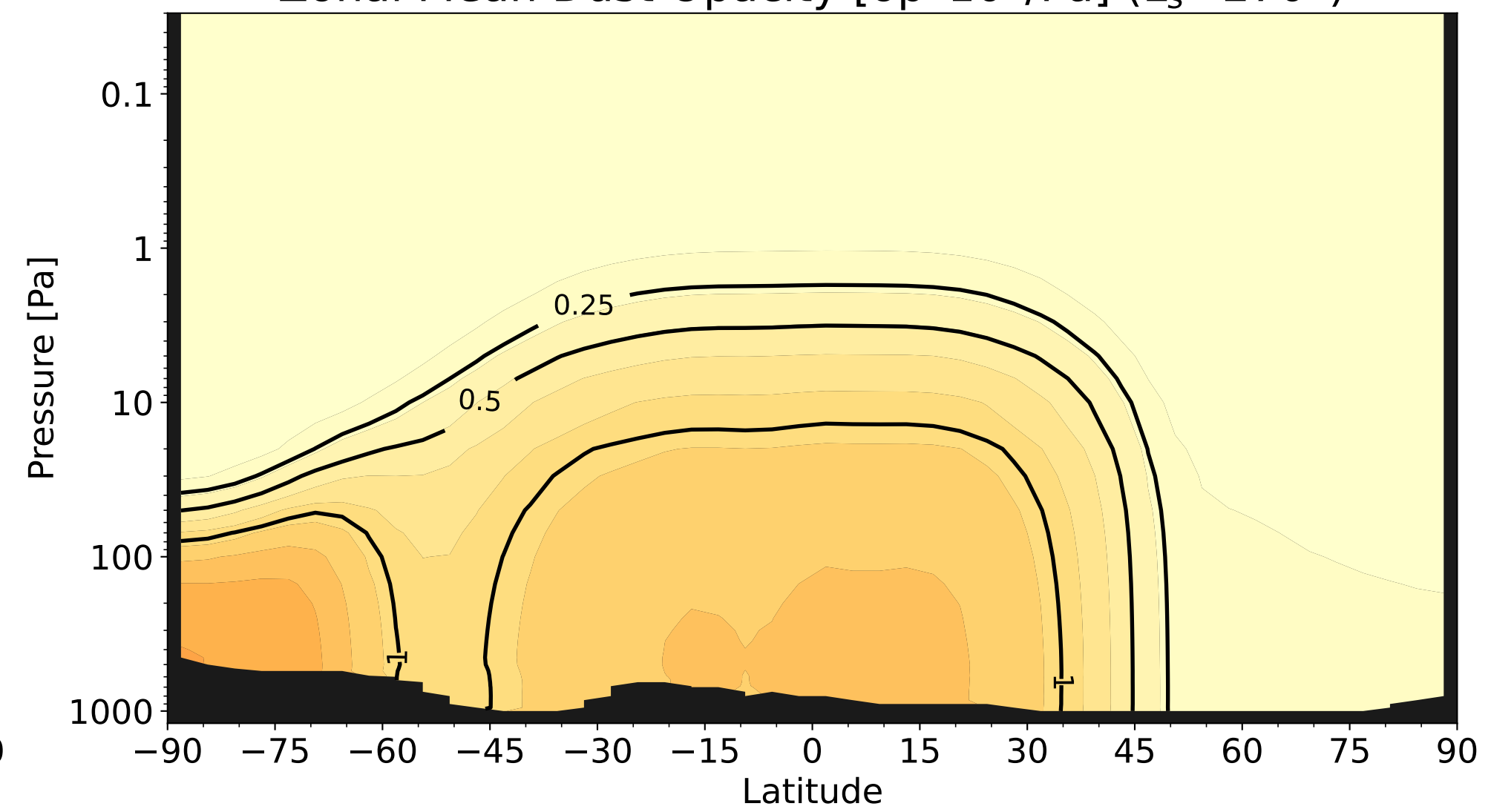
Zonal Mean Dust Opacity [ op \cdot 10^3 / Pa ] ( L_s=270^\circ )
