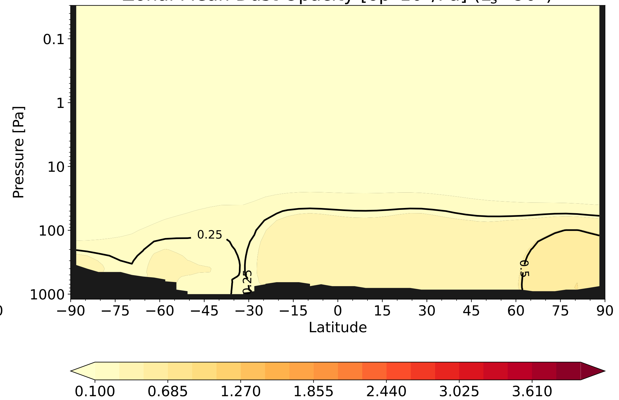
Zonal Mean Dust Opacity [ op \cdot 10^3 / Pa ] ( L_s=90^\circ )
