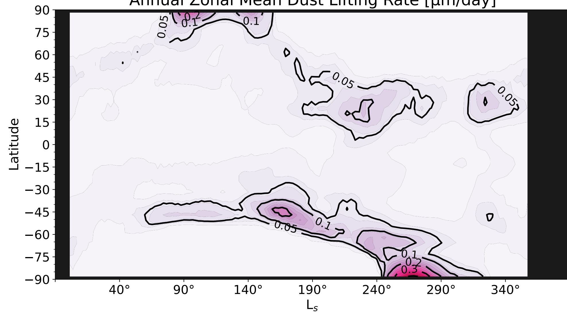
Annual Zonal Mean Dust Lifting Rate [ \mu\text{m/day} ]
