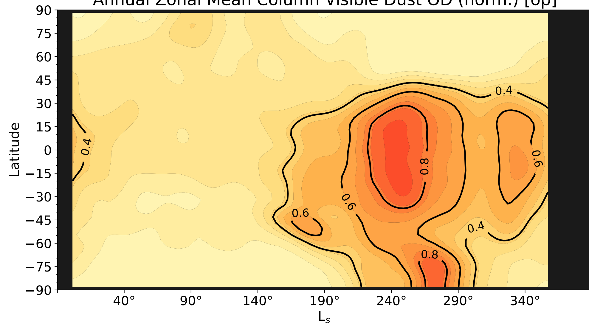
Annual Zonal Mean Column Visible Dust OD (norm.) [op]
