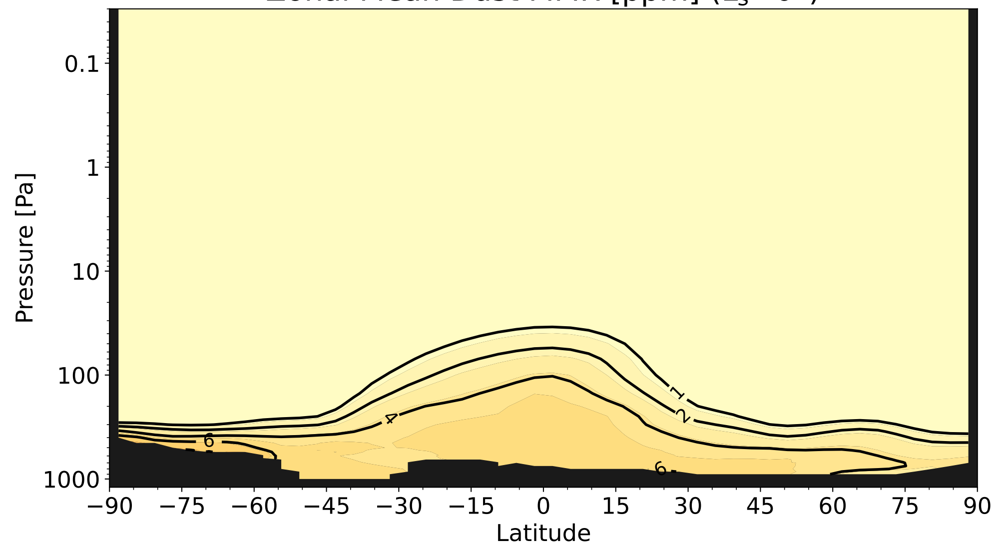
Zonal Mean Dust MMR [ppm] ( L_s=0^\circ )
