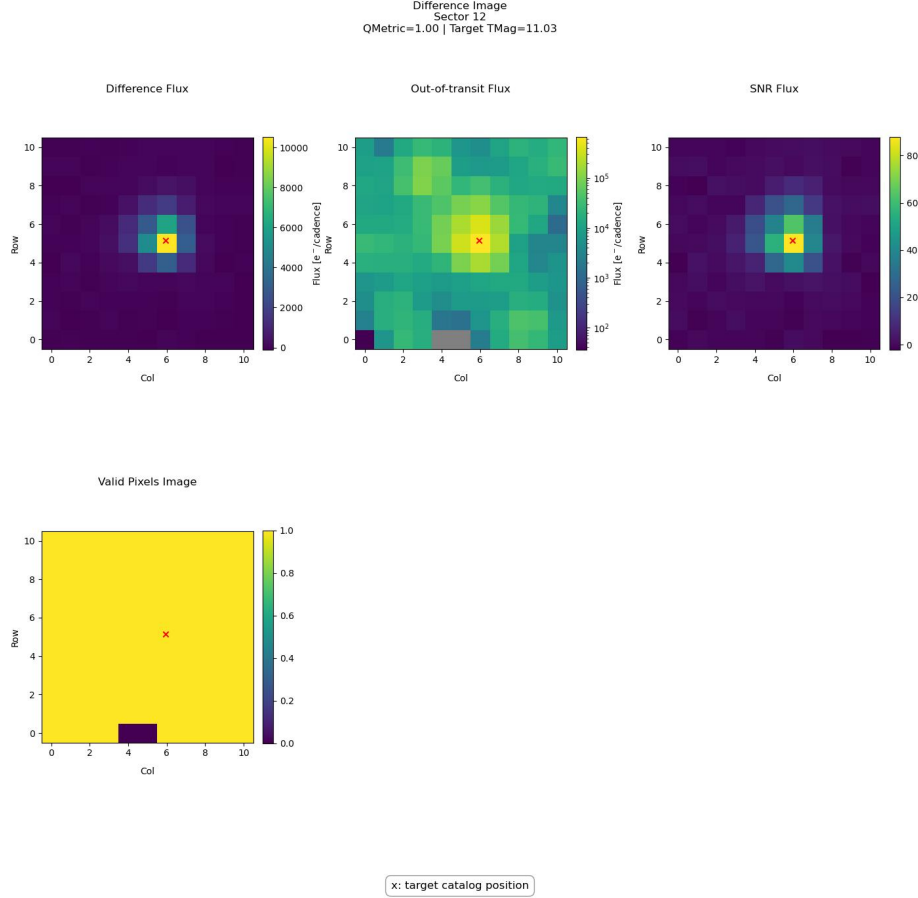
Figure 6: Difference image plots for TIC 66818296.1 in sector 12.
