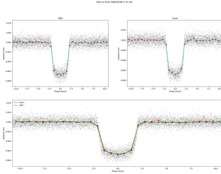
Figure 4: Odd-even plots for TIC 66818296.1.
