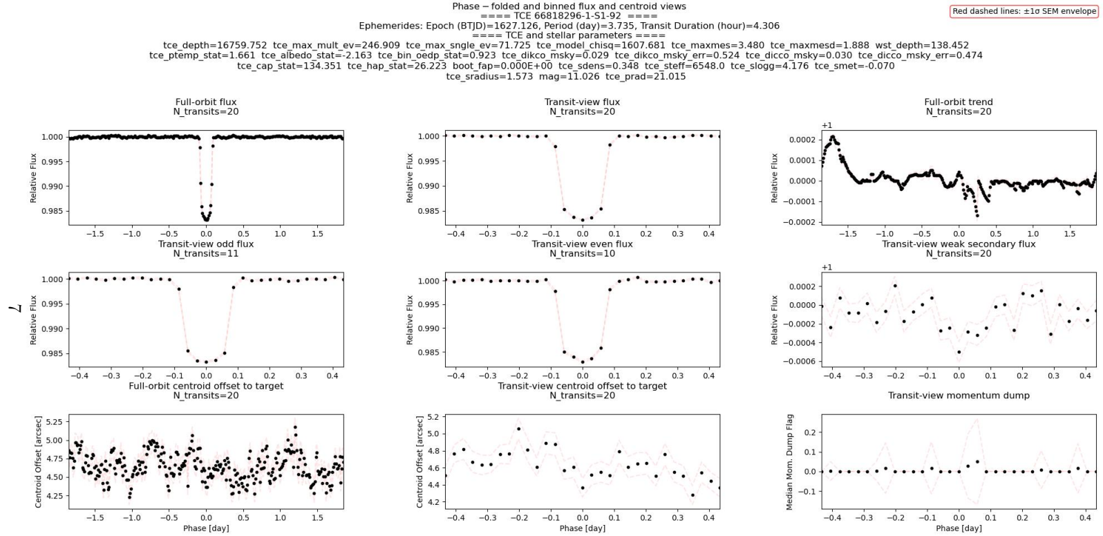
Figure 3: Phase-folded and binned flux and centroid plots for TIC 66818296.1.
