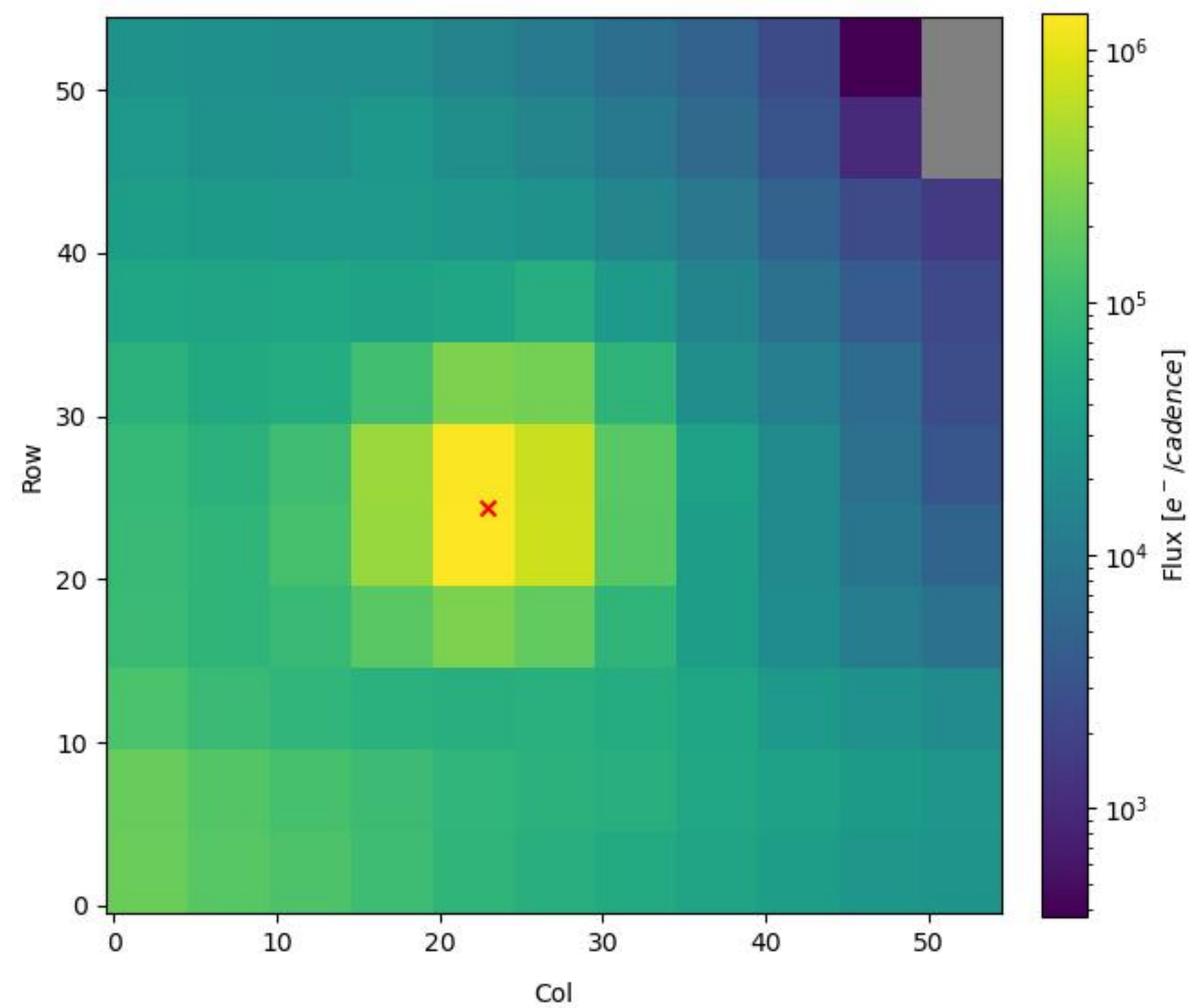
Out-of-transit Flux
