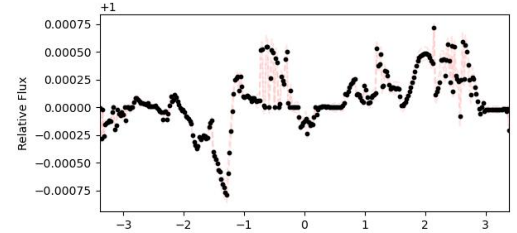
Full-orbit trend N_transits=13
