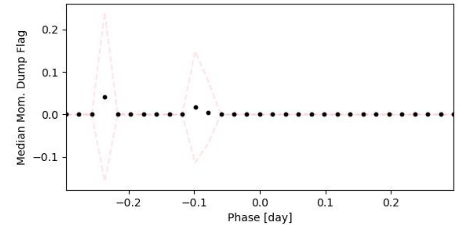
Transit-view momentum dump
