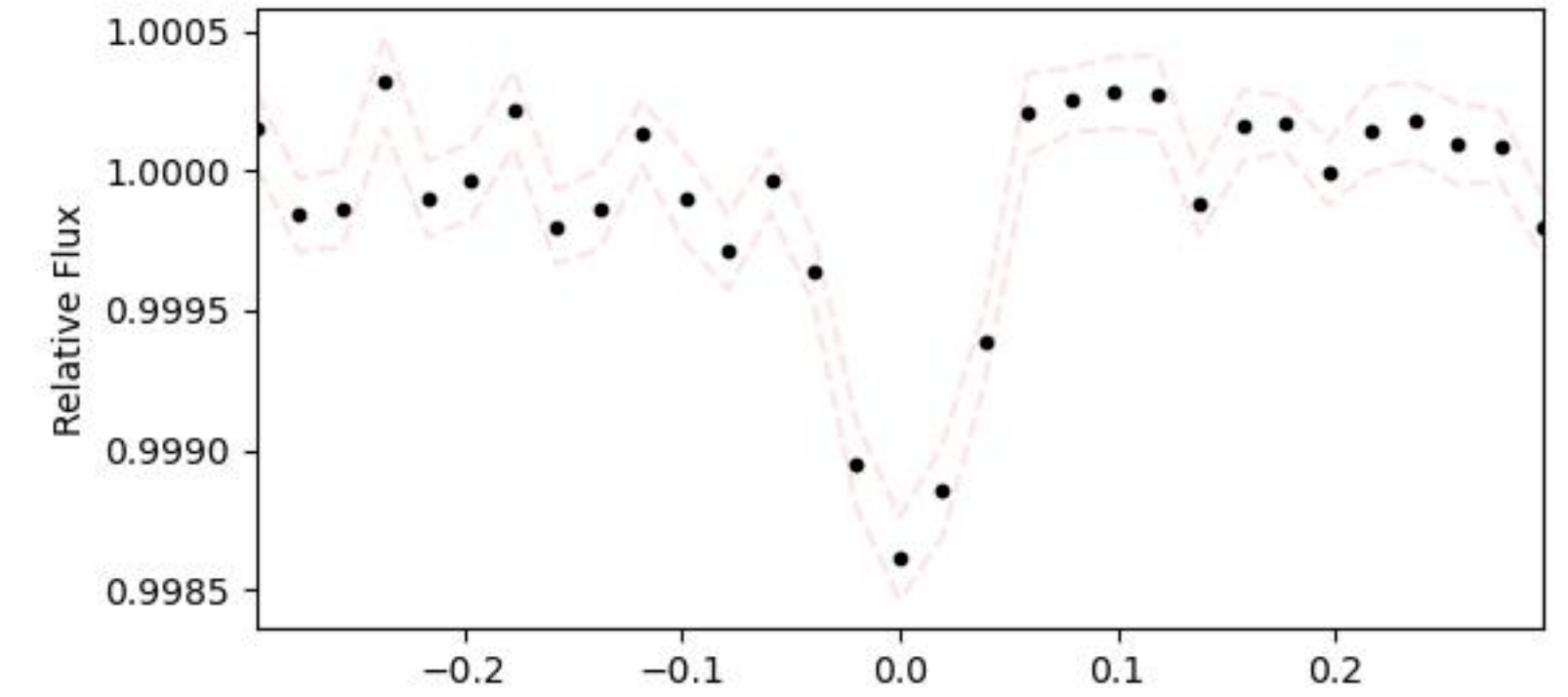
Transit-view weak secondary flux N_transits=13
