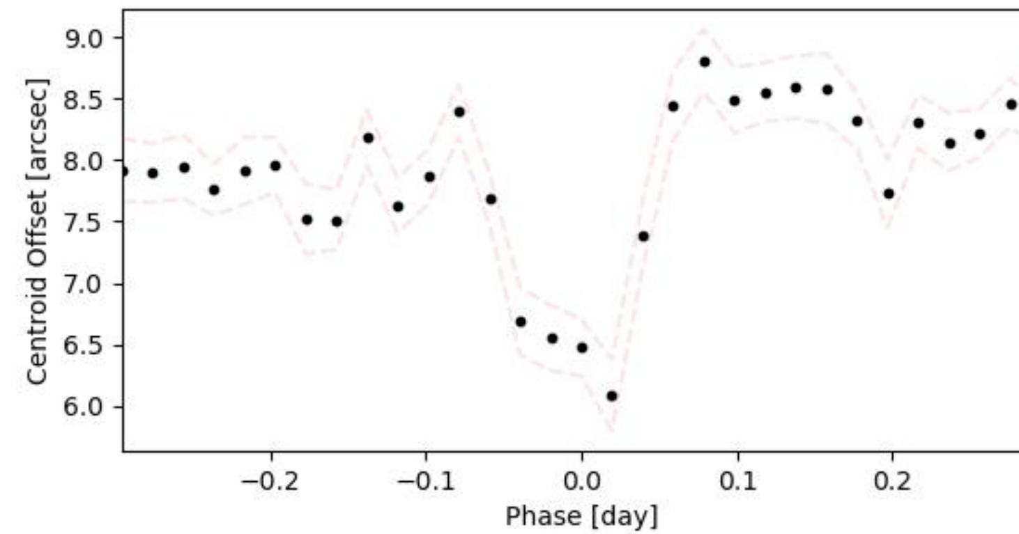
Transit-view centroid offset to target N_transits=13
