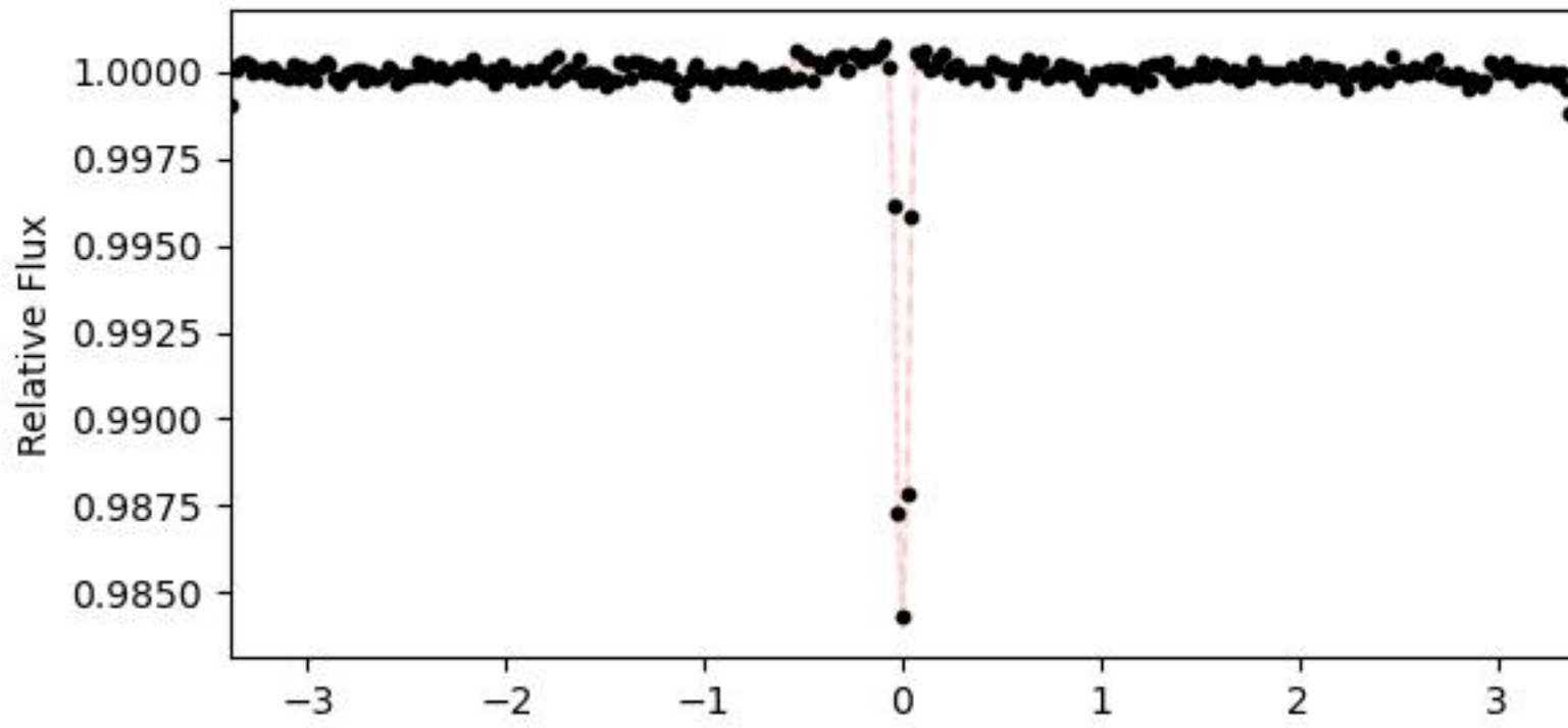
Transit-view odd flux N_transits=7
