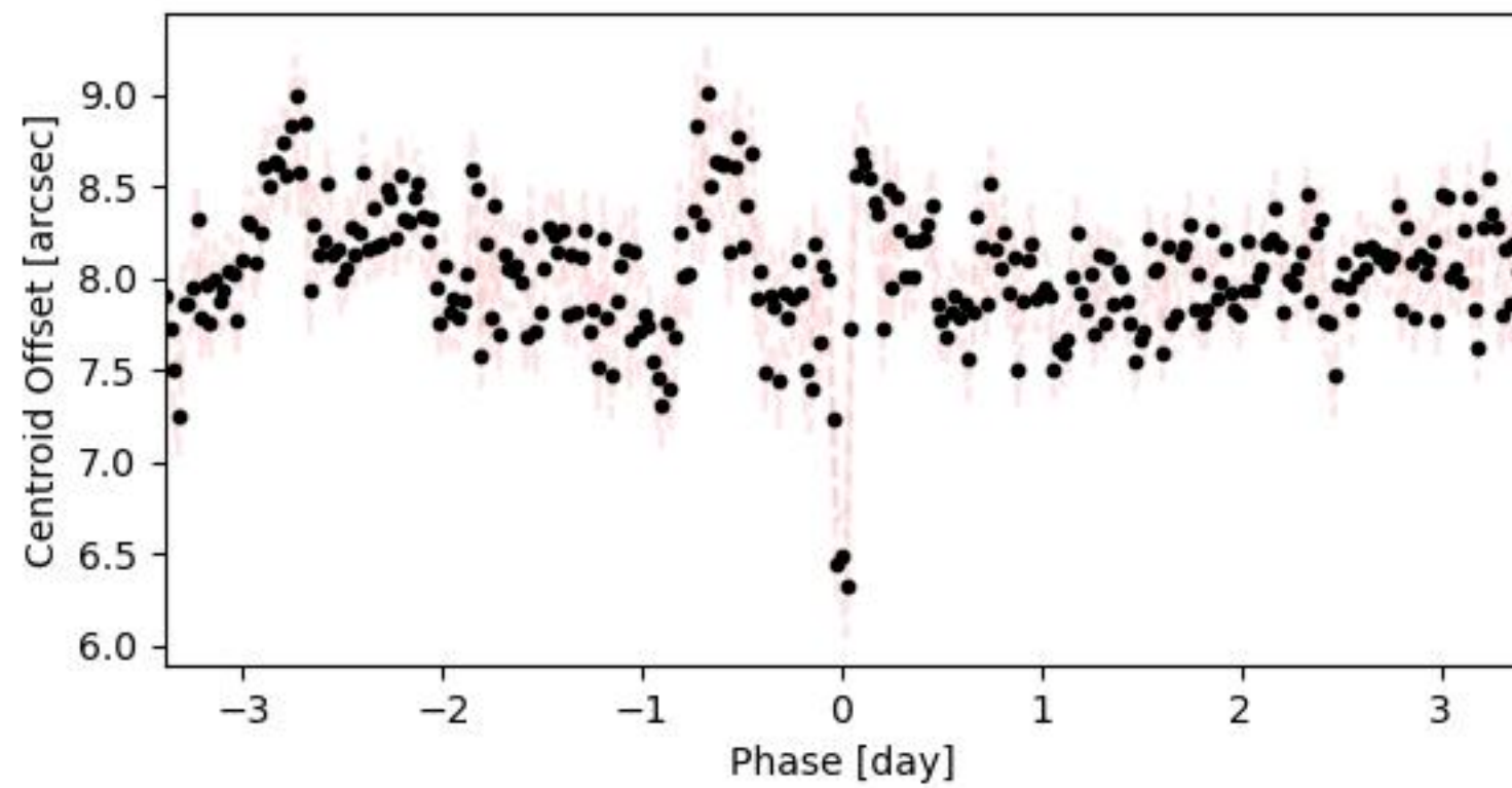
Full-orbit centroid offset to target N_transits=13
