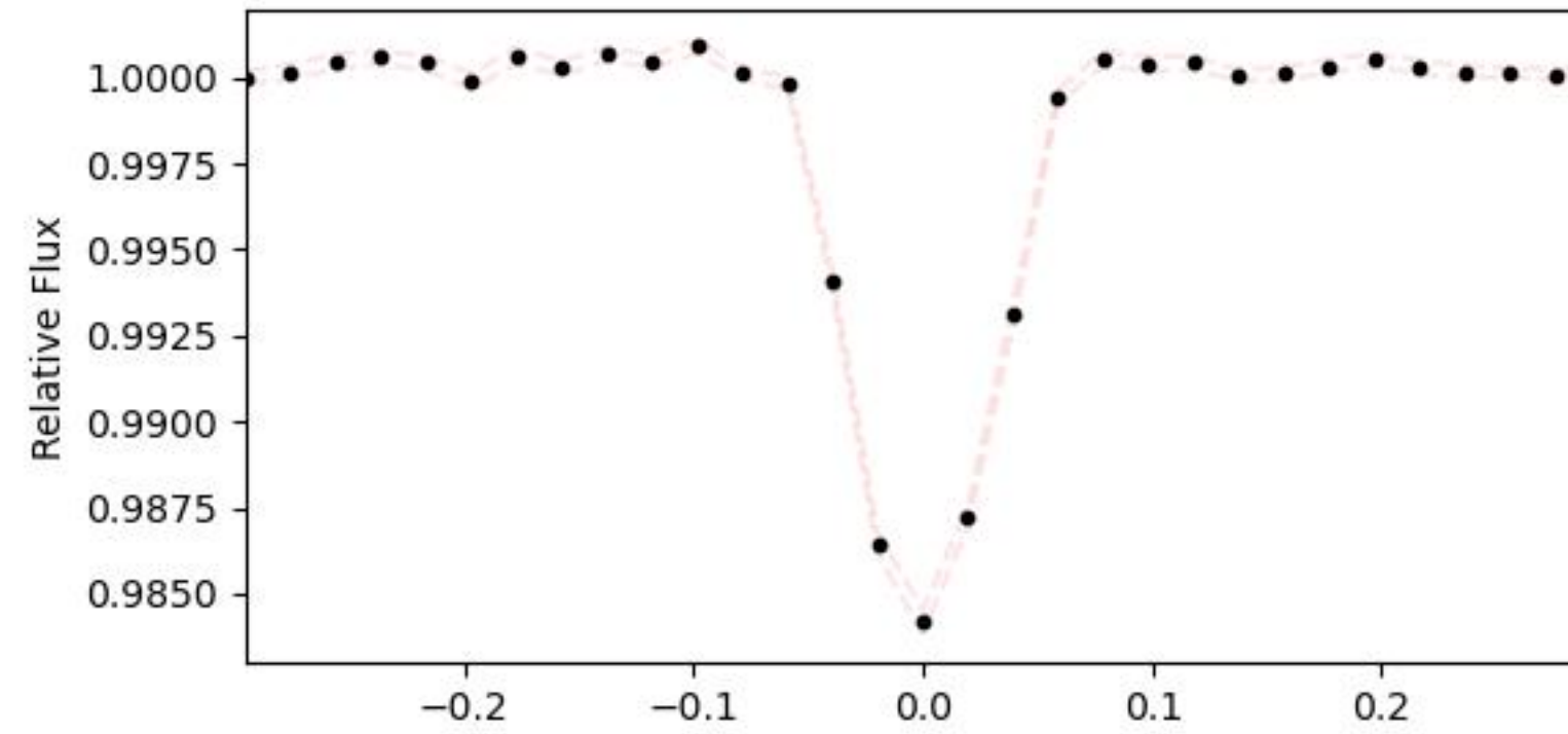
Transit-view even flux N_transits=8
