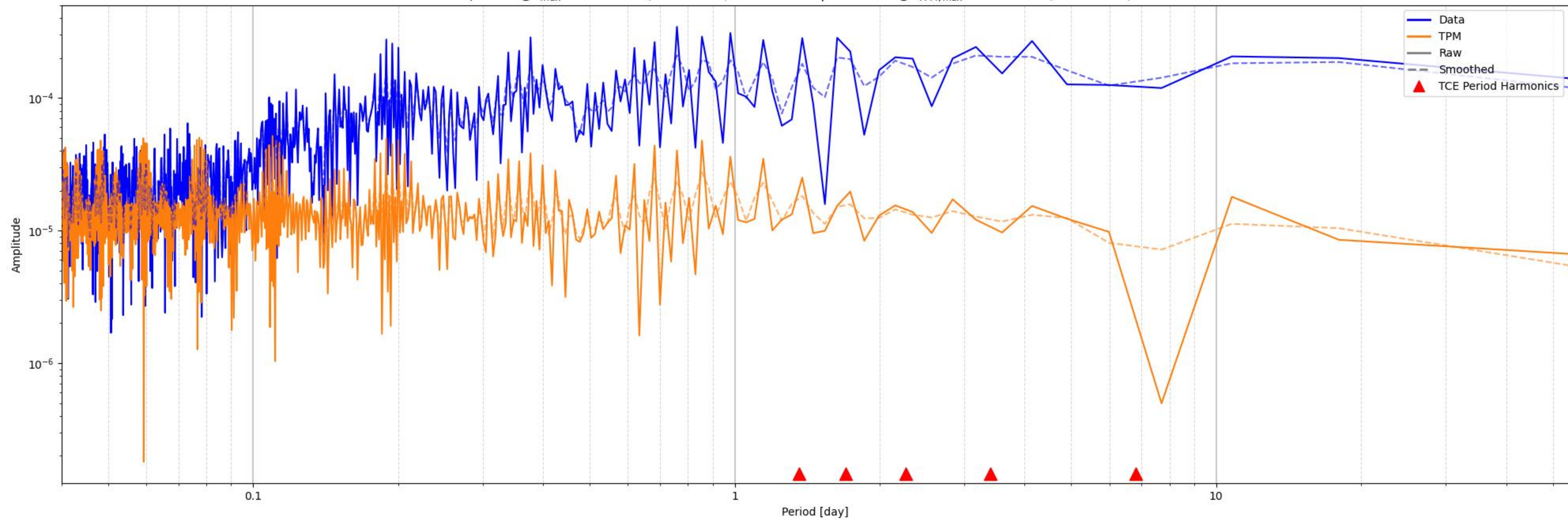
Periodogram TCE 347538174-1-S14-86 | Period: 6.803 day Peak Amplitude @ f_{max} = 1.318 \text{ d}^{-1} ( P = 0.759 \text{ d} ): 3.444e-04 | TPM Peak @ f_{TPM,max} = 9.113 \text{ d}^{-1} ( P = 0.110 \text{ d} ): 5.165e-05
