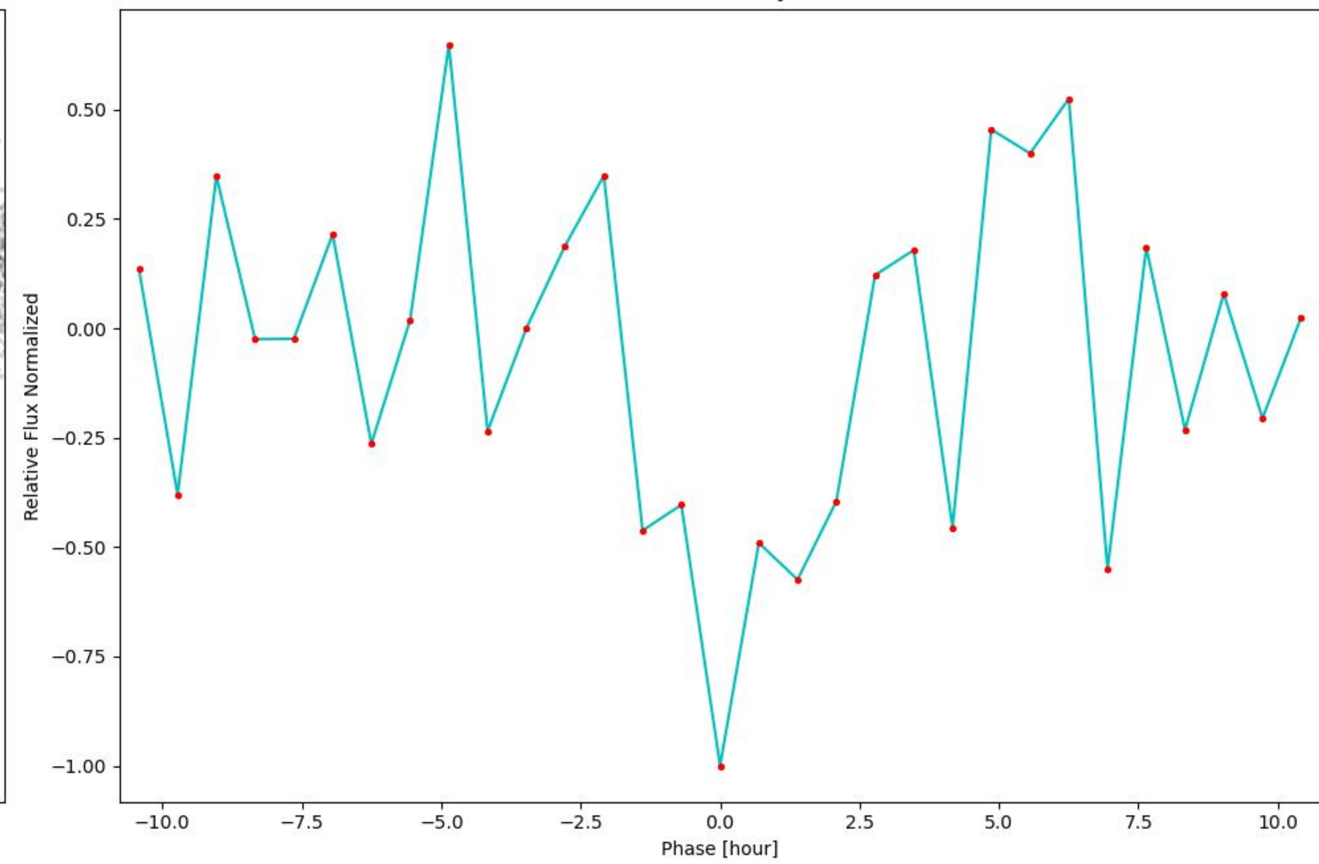
Transit-View Normalized by Abs. Min. Flux
