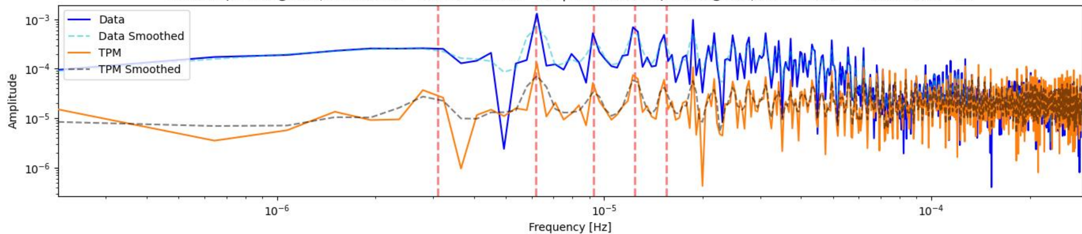
Peak Amplitude @ f_{Data,max} = 6.229e - 061/s = 1.302e - 03 | TPM Peak Amplitude @ f_{TPM,max} = 6.229e - 061/s:1.302e - 04
