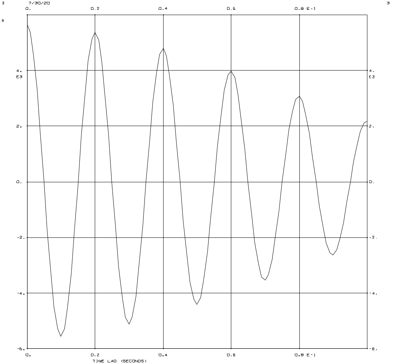
AUTOCORRELATION FUNCTION FOR POINT 6 DISPLACEMENT FREQUENCY RESPONSE AND RANDOM ANALYSIS OF A 10 CELL BEAM NASTRAN DEMONSTRATION PROBLEM NO. D11-D1-1A
