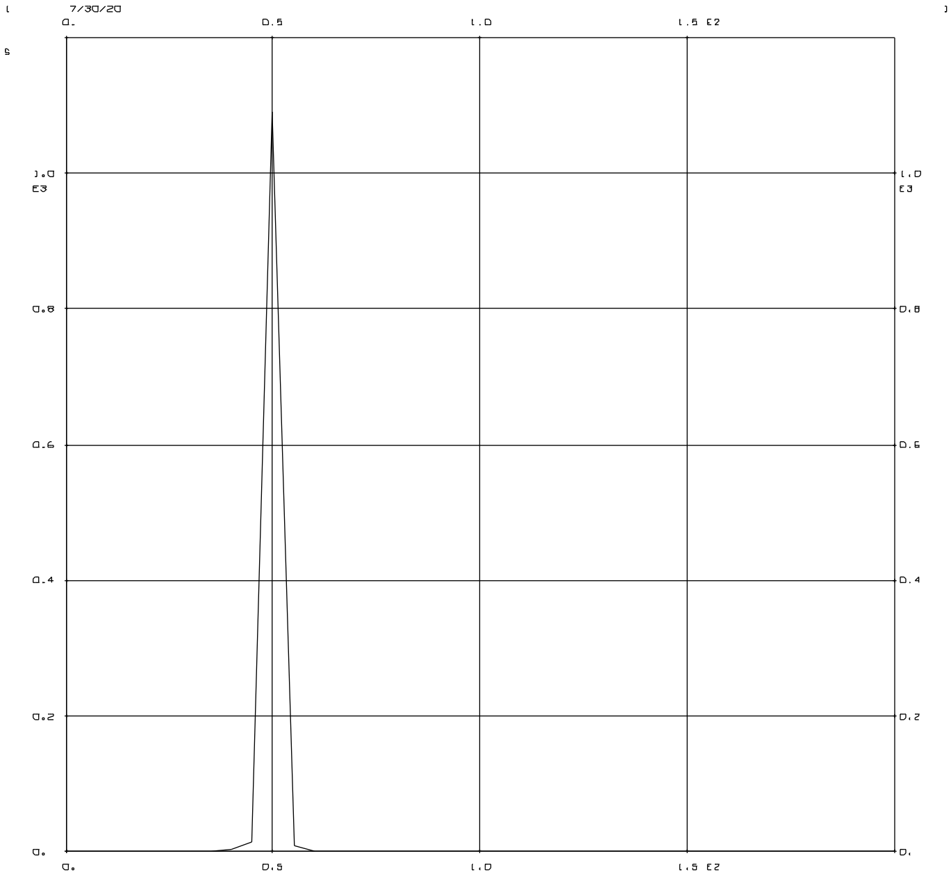
POWER SPECTRAL DENSITY OF POINT 6 DISPLACEMENT FREQUENCY RESPONSE AND RANDOM ANALYSIS OF A 10 CELL BEAM NASTRAN DEMONSTRATION PROBLEM NO. D11-D1-1A
