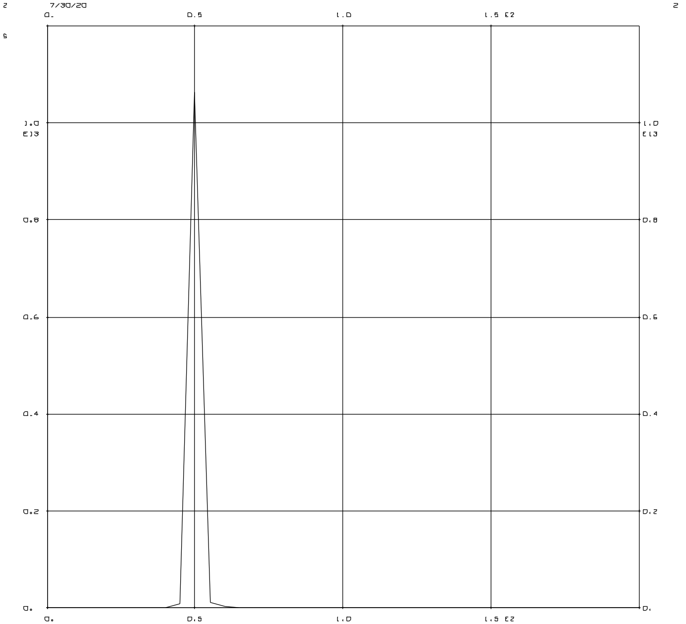
POWER SPECTRAL DENSITY OF POINT 6 ACCELERATION FREQUENCY RESPONSE AND RANDOM ANALYSIS OF A 10 CELL BEAM NASTRAN DEMONSTRATION PROBLEM NO. D11-D1-1A
