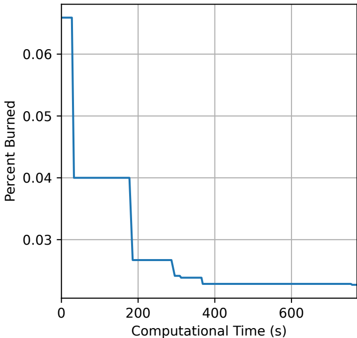
Progression of Direct Algorithm Over Time
