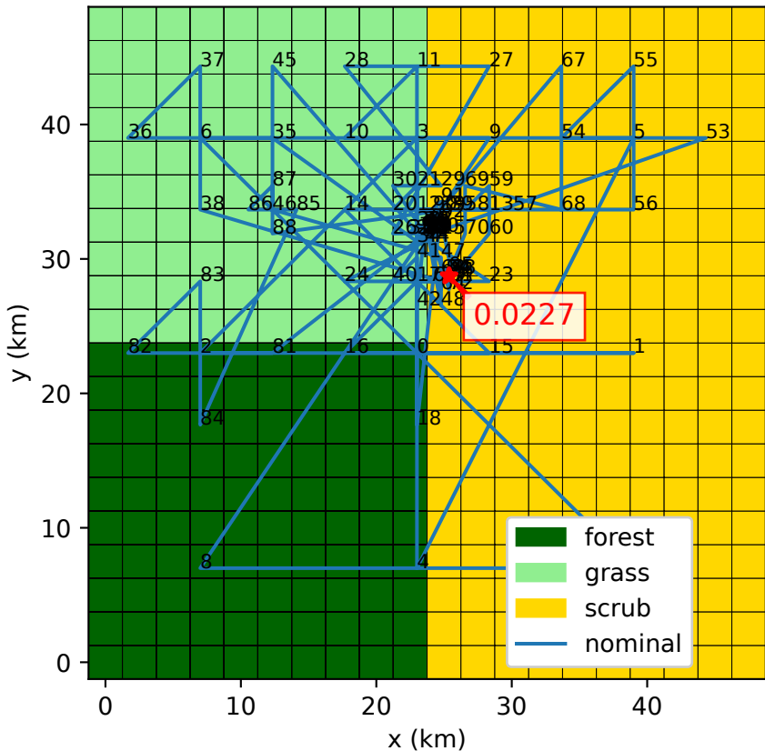
Progression of DIRECT Algorithm Over Map
